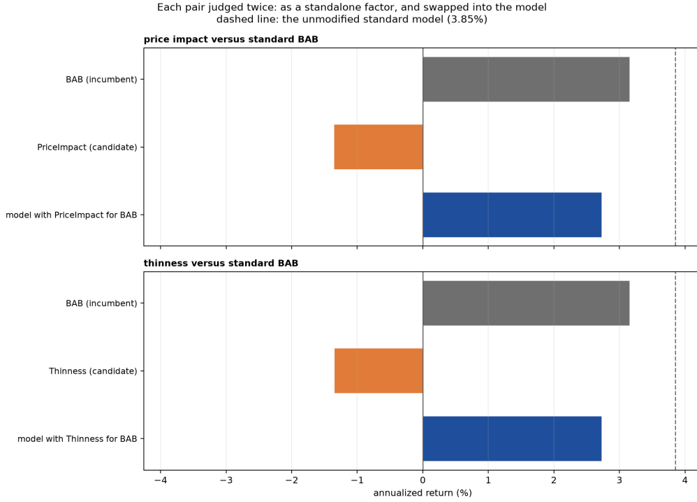
Figure 7: Each pair judged twice: the incumbent factor against the candidate standing alone, then the model with the candidate swapped in. The dashed line is the unmodified standard model.
