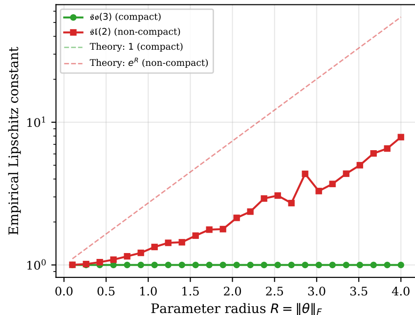
(c) Smoothness dichotomy: compact vs. non-compact
