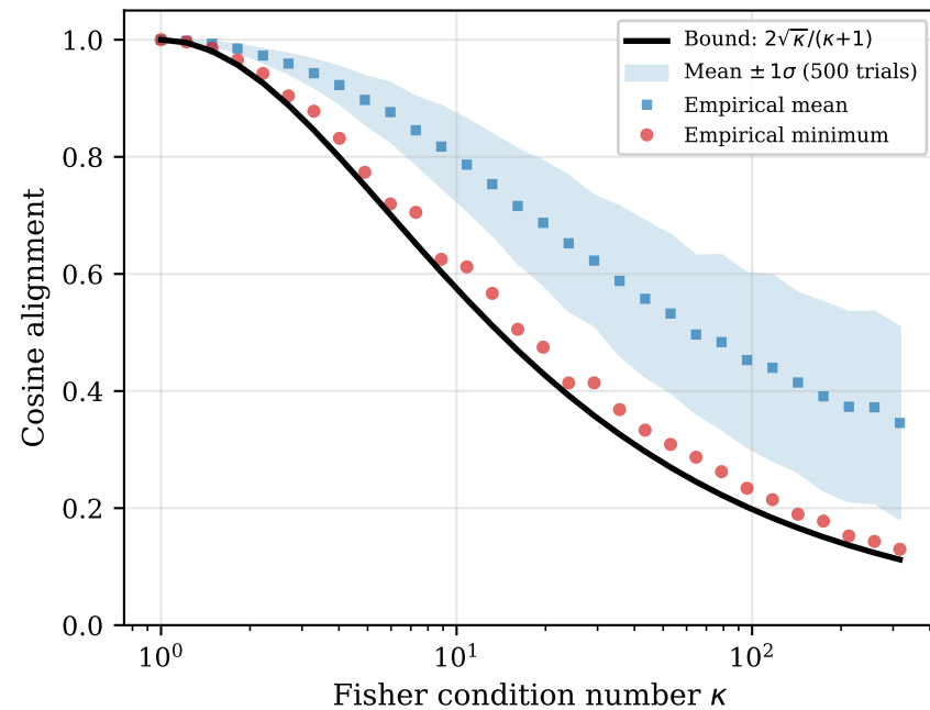
(a) Alignment bound tightness
