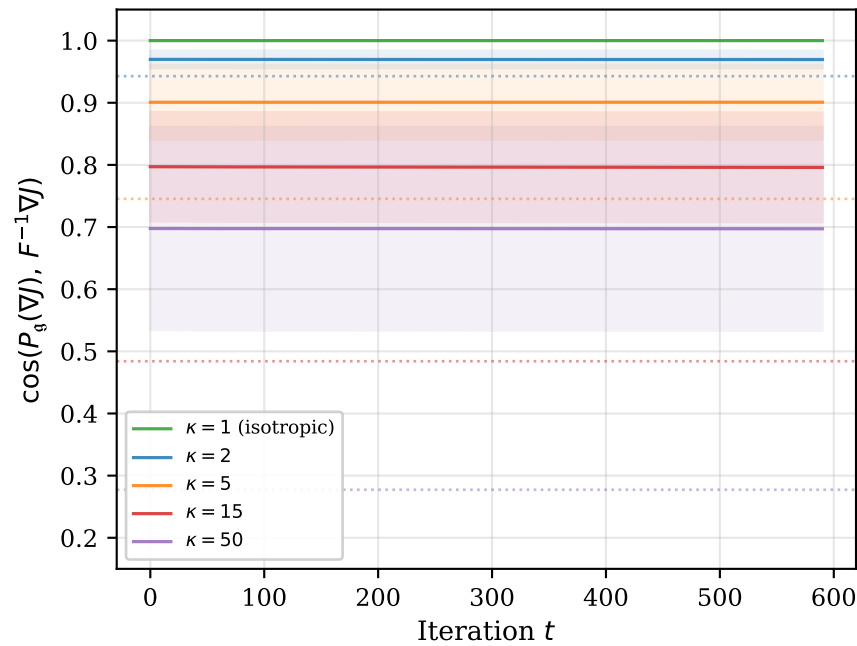
(b) Alignment during optimization on \mathfrak{so}(3)
