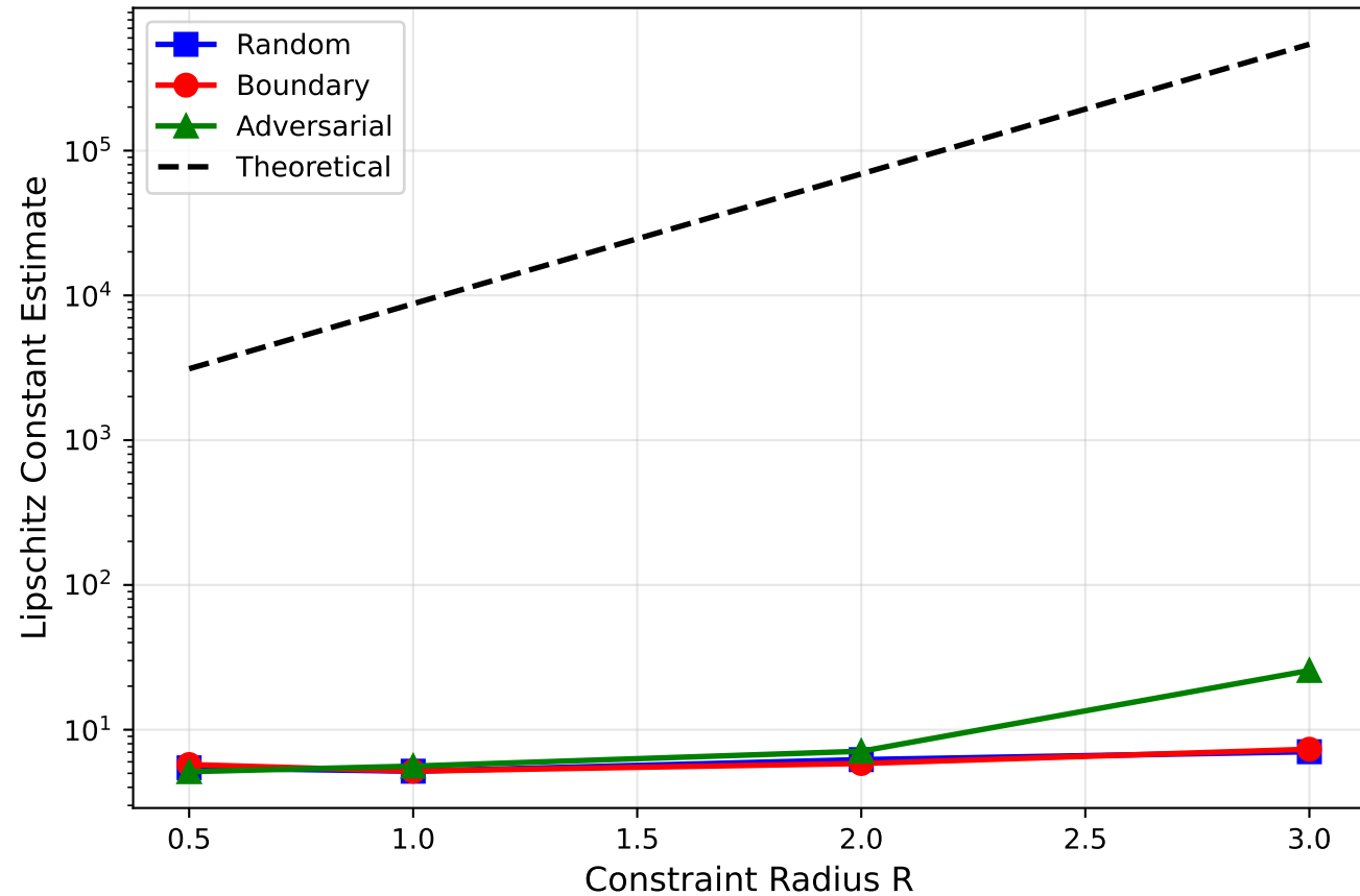
Empirical vs Theoretical Lipschitz on sl(12)
