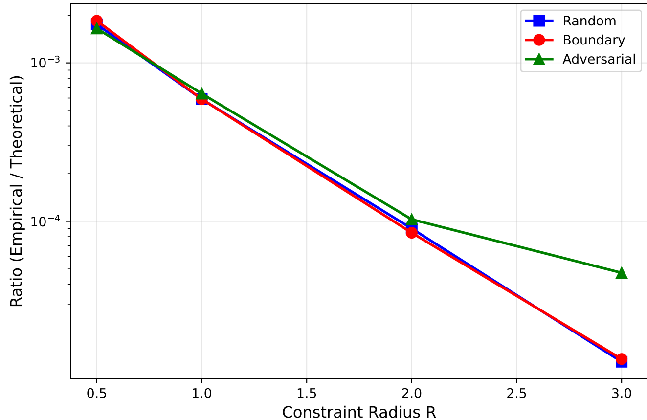
Tightness of Bounds by Sampling Strategy
