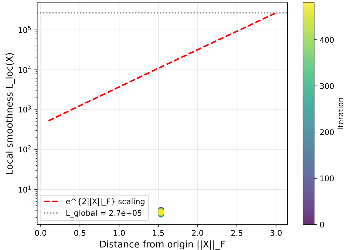
Local Smoothness on sl(16) with R=3.0
