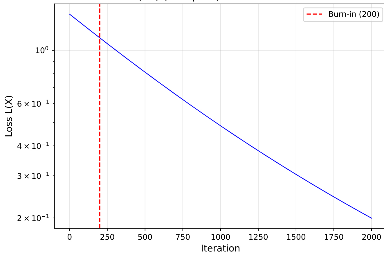
so(16) (Compact): Loss vs Iteration
