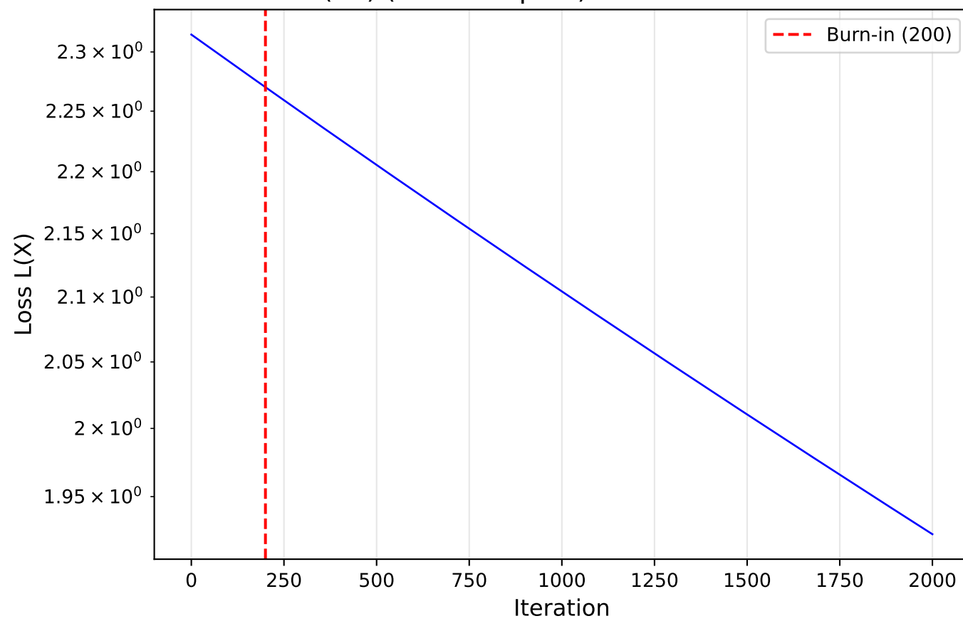
sl(16) (Non-Compact): Loss vs Iteration
