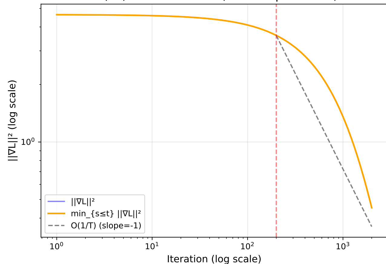
sl(16): Gradient Norm (fitted slope: -0.127)
