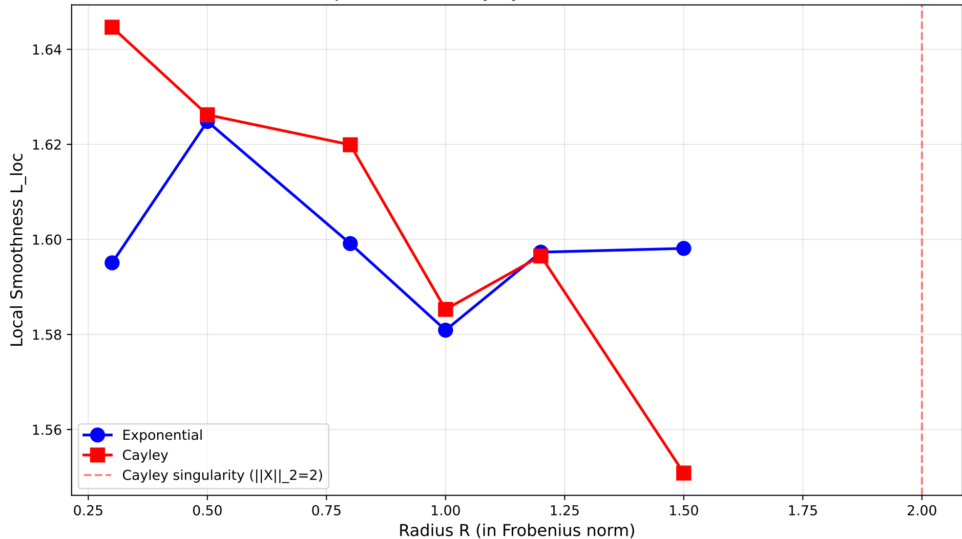
Exponential vs Cayley Retraction on so(16)
