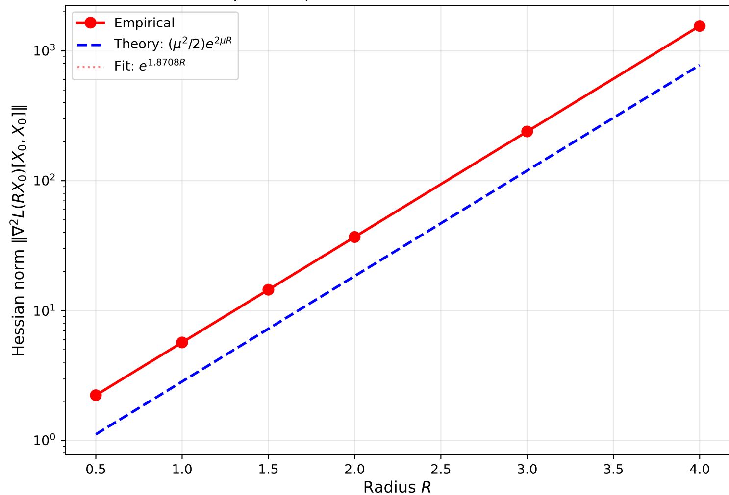
Lower Bound Verification on \mathfrak{sl}(8) Empirical exponent: 1.8708, Theoretical: 1.8708
