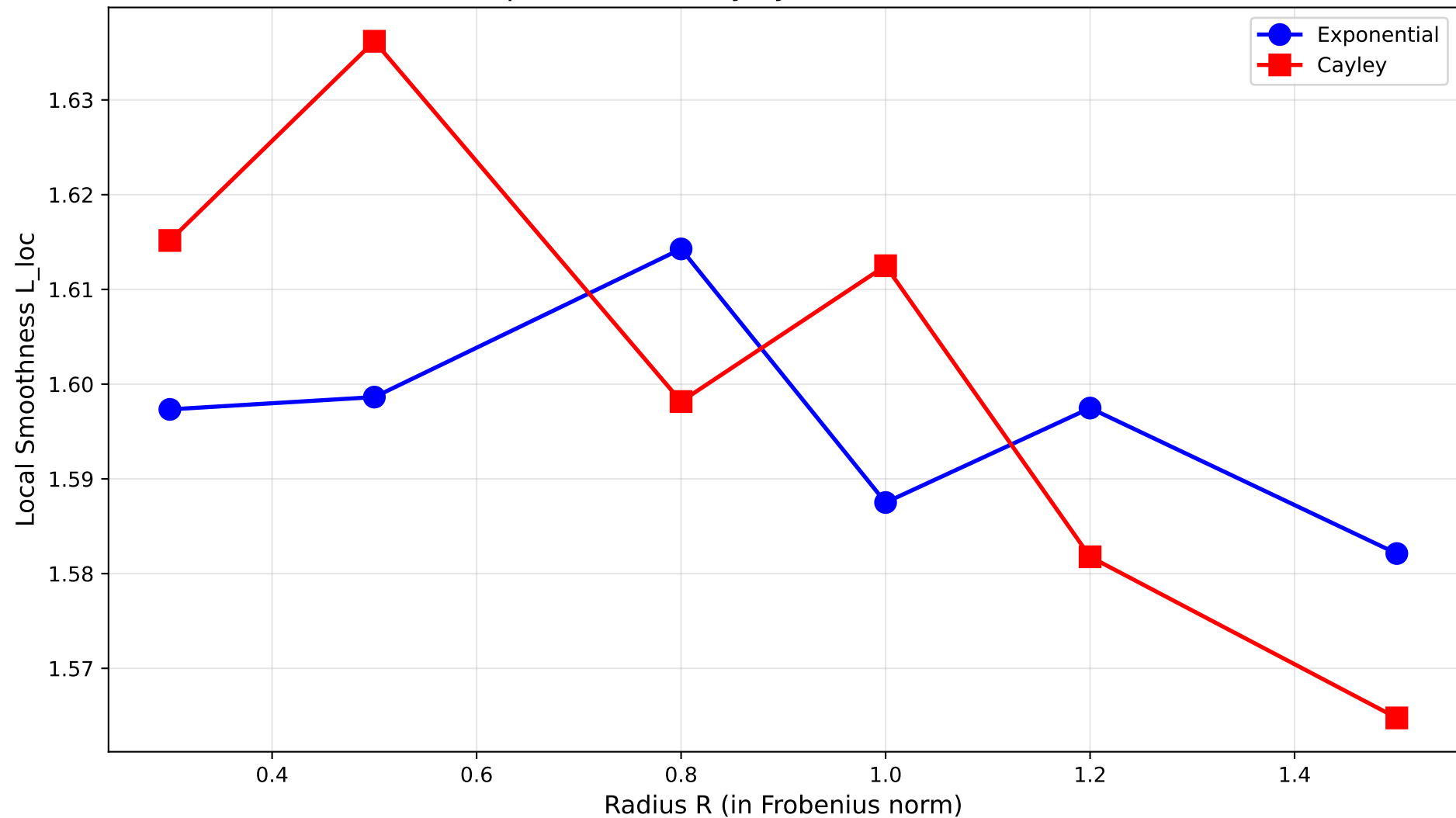
Exponential vs Cayley Retraction on \mathfrak{so}(16)
