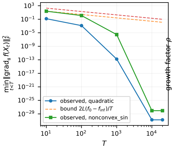
Stationarity rate at \eta = 1/L
