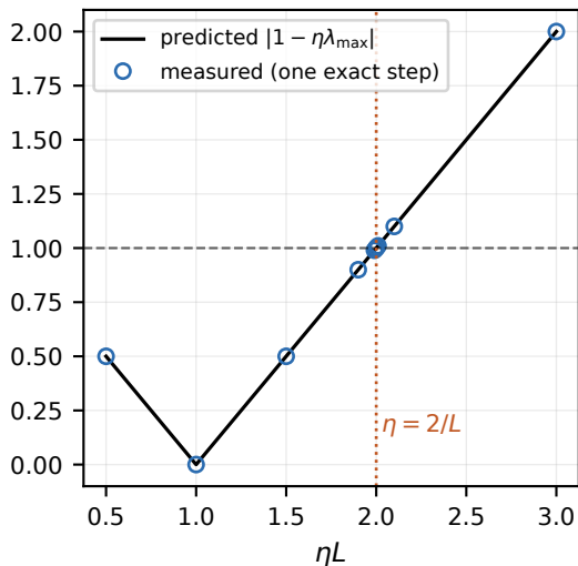
Sharp divergence threshold
