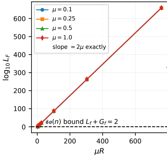
Exponential curvature on a non-compact direction
