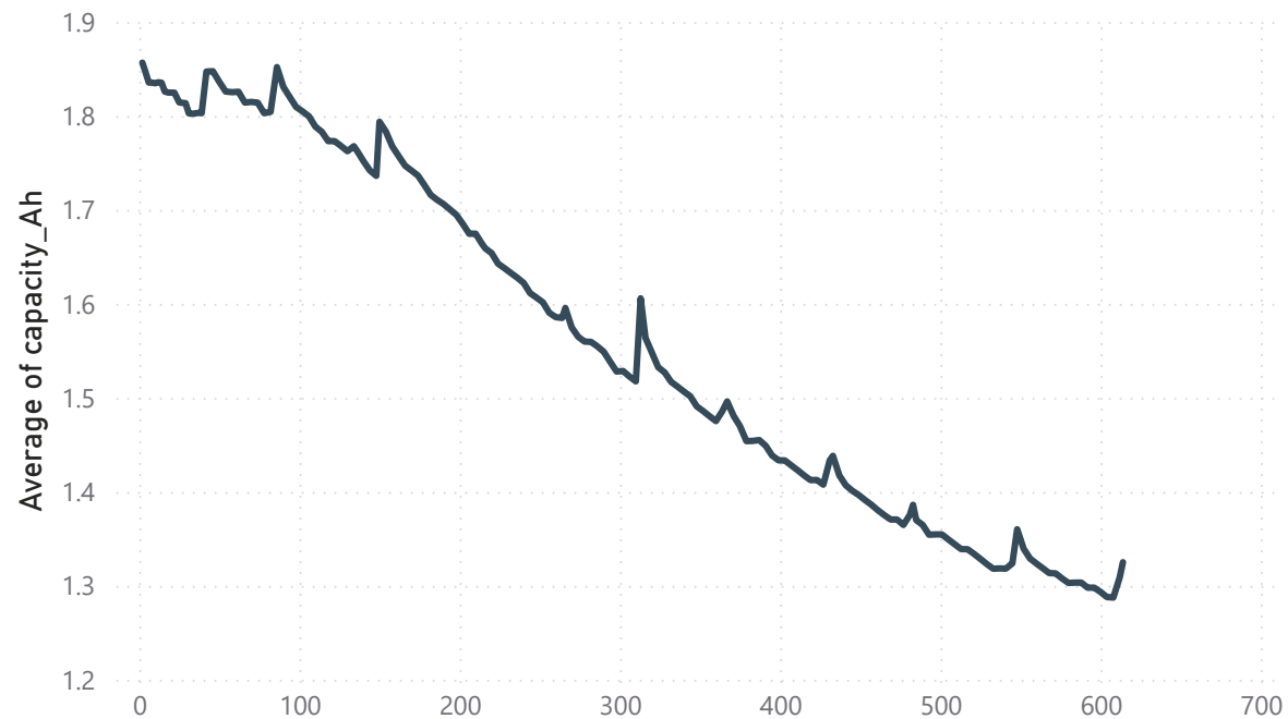
Average of capacity_Ah by cycle_index
