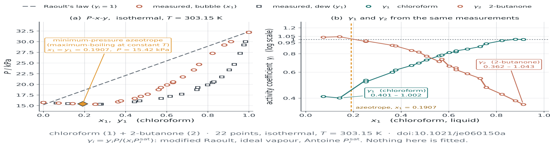
Type 3 — negative deviation — maximum-boiling azeotrope
