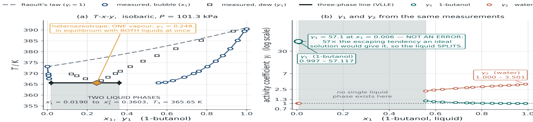
Type 4 — VLLE — partial miscibility, heteroazeotrope
