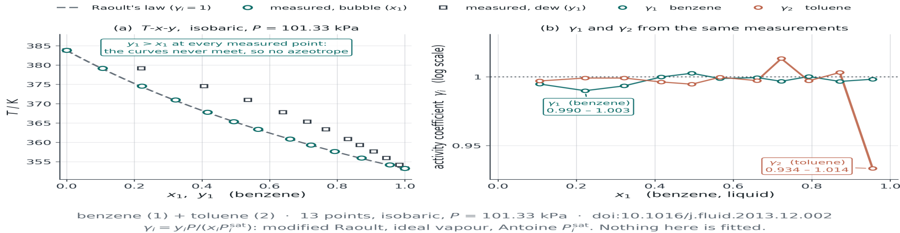
Type 1 — ideal solution — \gamma_i \approx 1 , no azeotrope
