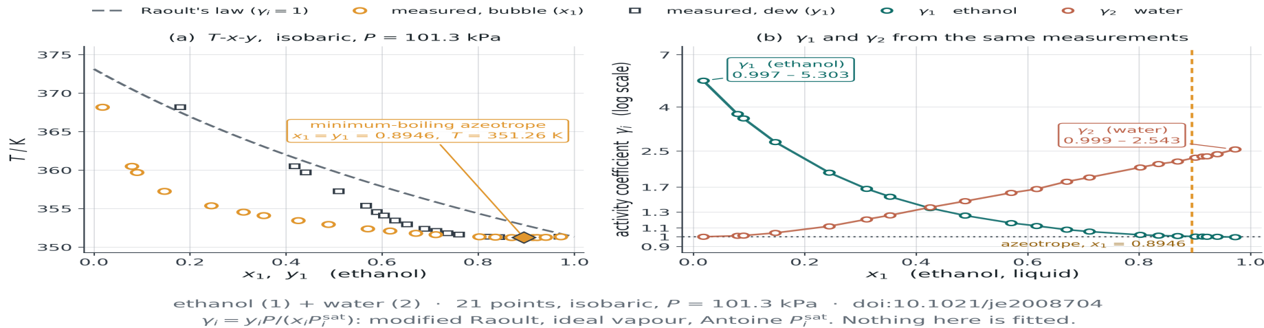
Type 2 — positive deviation — minimum-boiling azeotrope
