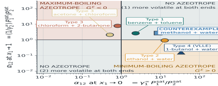
(a) the criterion as a map: an azeotrope exists iff \alpha_{12} straddles 1
