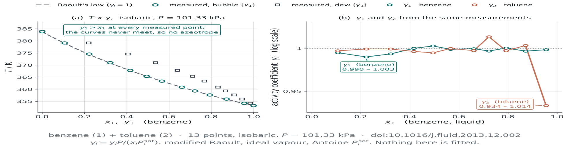
Type 1 — ideal solution — \gamma_i \approx 1 , no azeotrope
