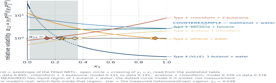
(b) the same statement in composition space
