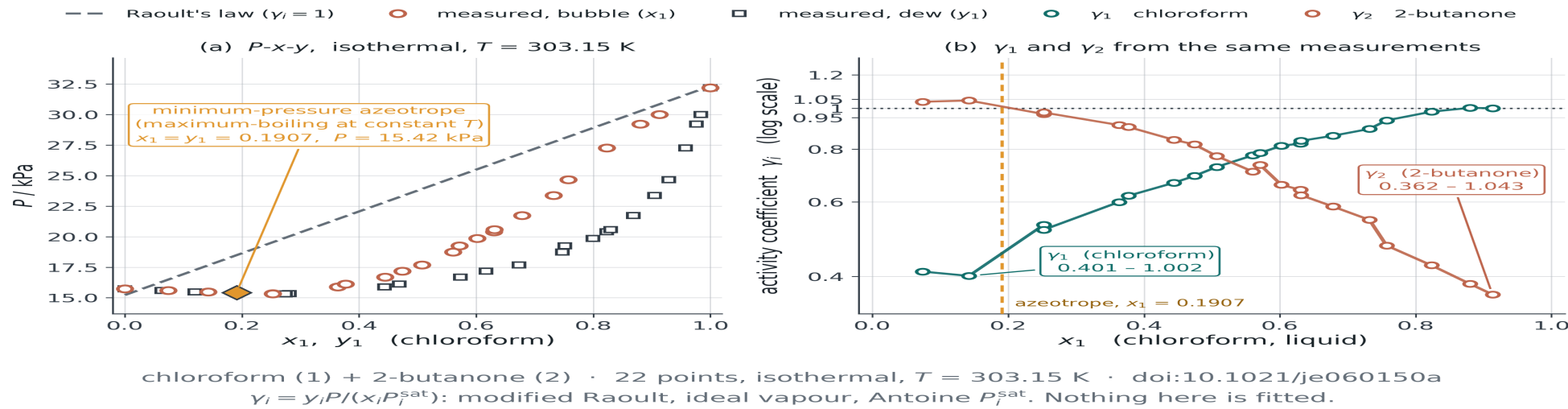
Type 3 — negative deviation — maximum-boiling azeotrope
