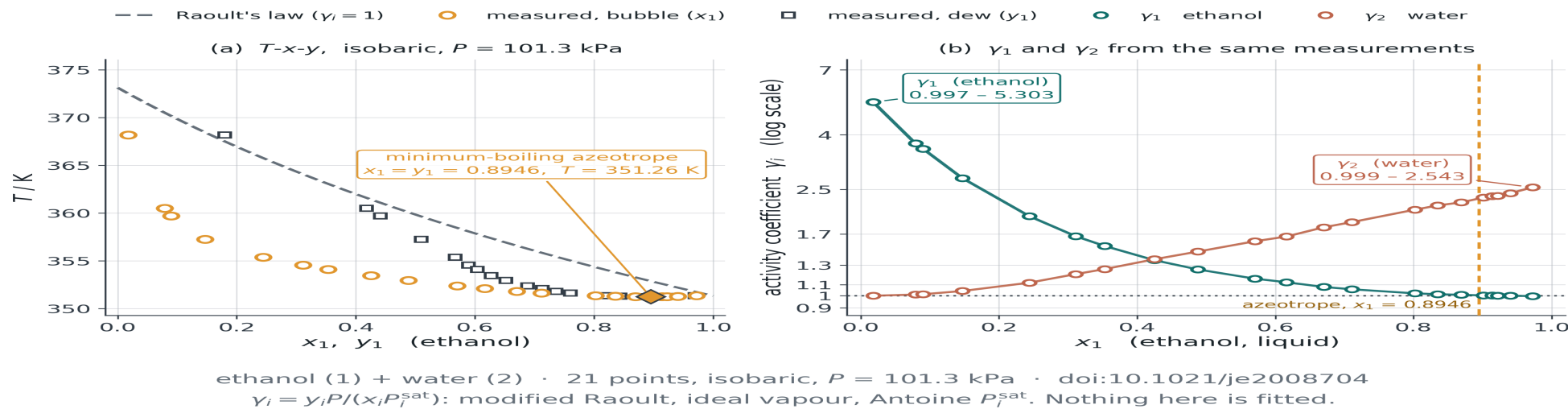
Type 2 — positive deviation — minimum-boiling azeotrope
