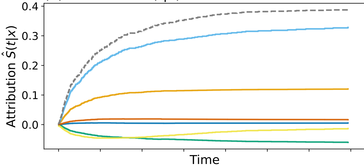
(7) GT: General Additive G(t|x) TD Main
