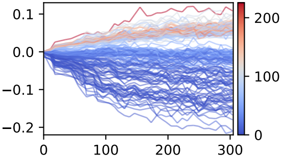
cd4 (order 1)
