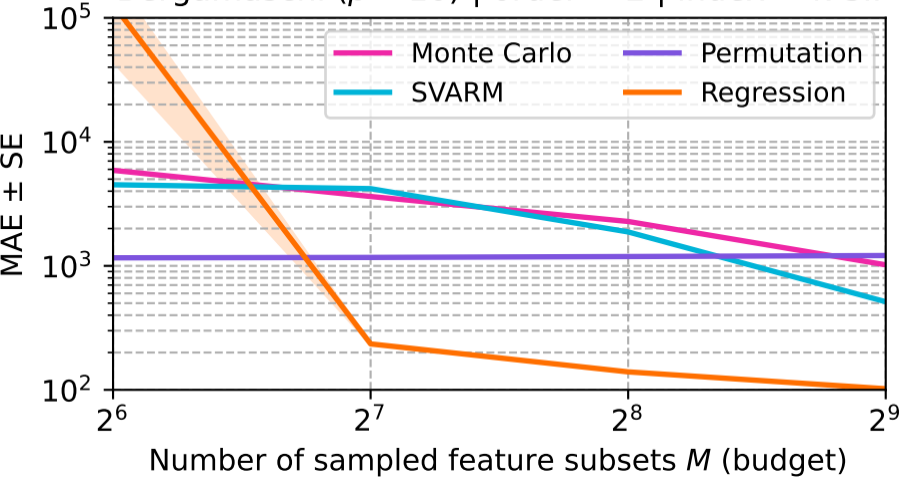
Bergamaschi ( p = 10 ) | order = 2 | index = k-SII
