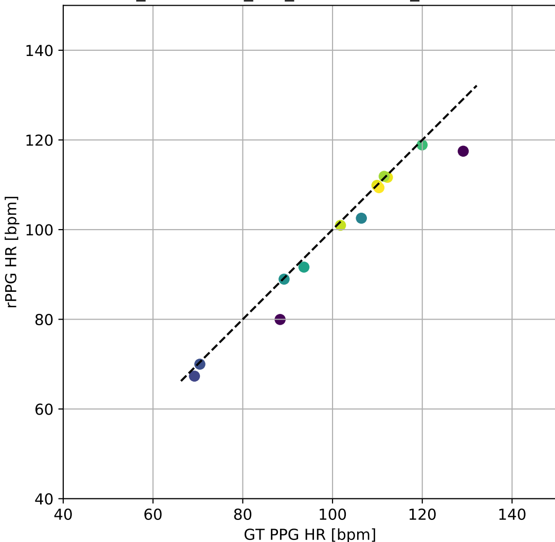
POS_UBFC-rPPG_FFT_BlandAltman_ScatterPlot
