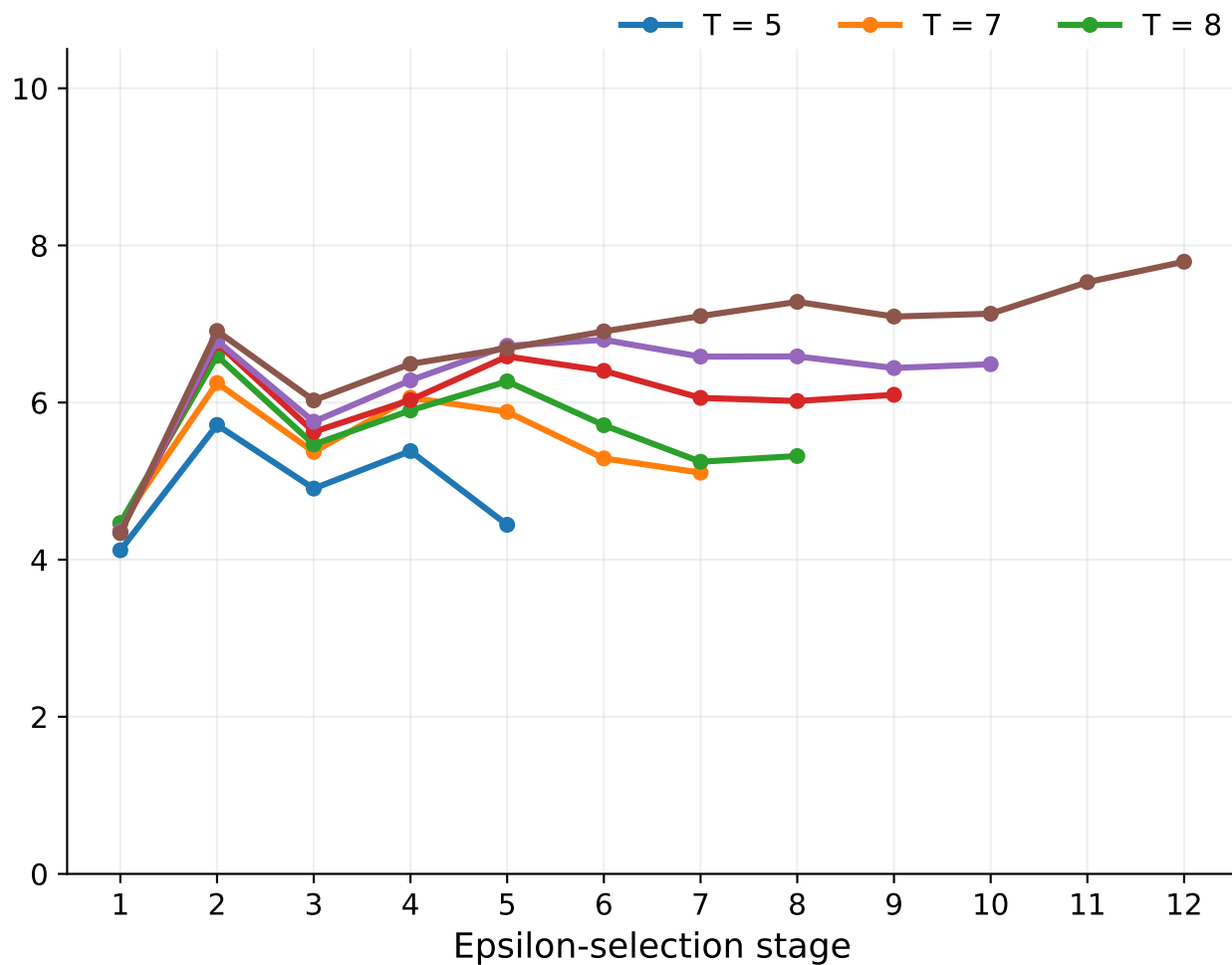
Mean number of admissible treatments
