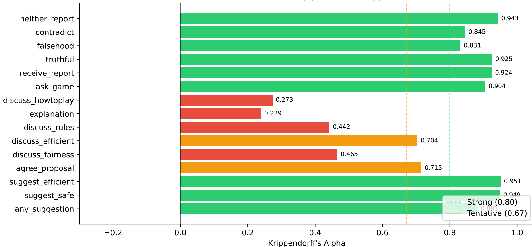
Human Inter-Rater Reliability per Label (Krippendorff's \alpha )
