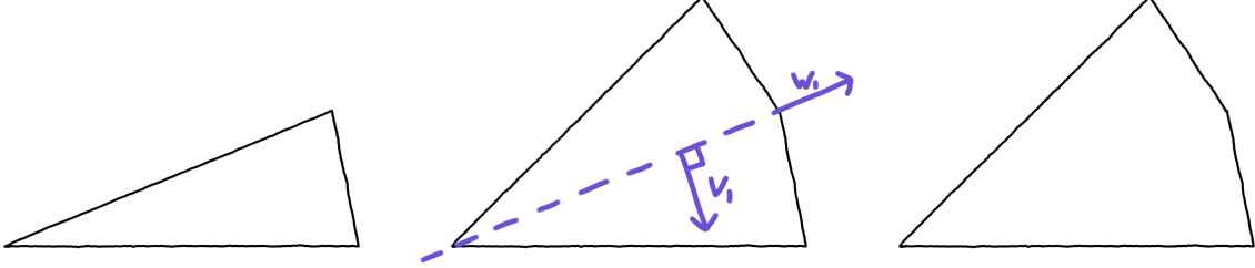
Figure 6: Left: P_1 for k = 4 . Middle: we double the triangle. Right: P_2 .
