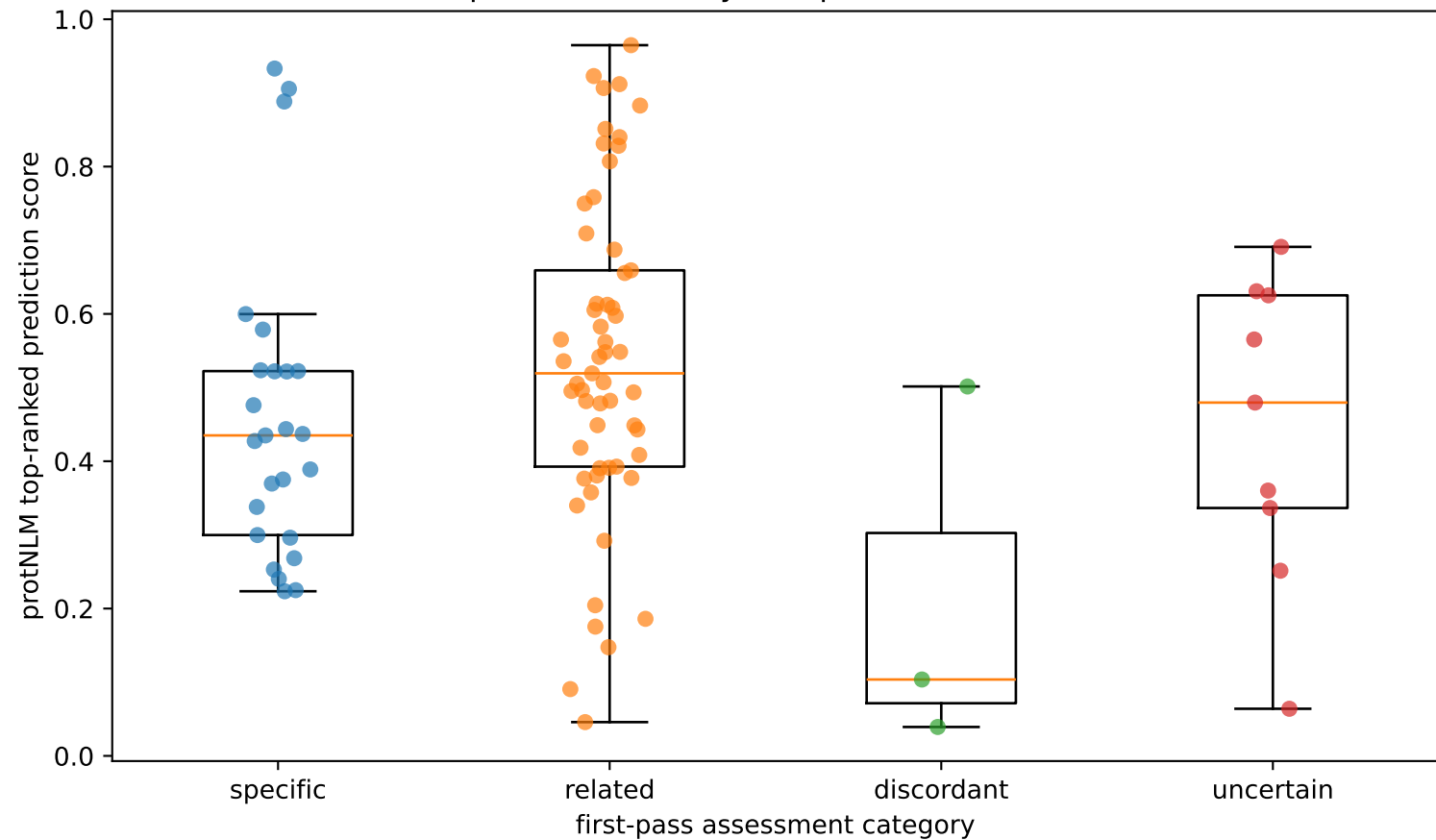
protNLM score by first-pass assessment
