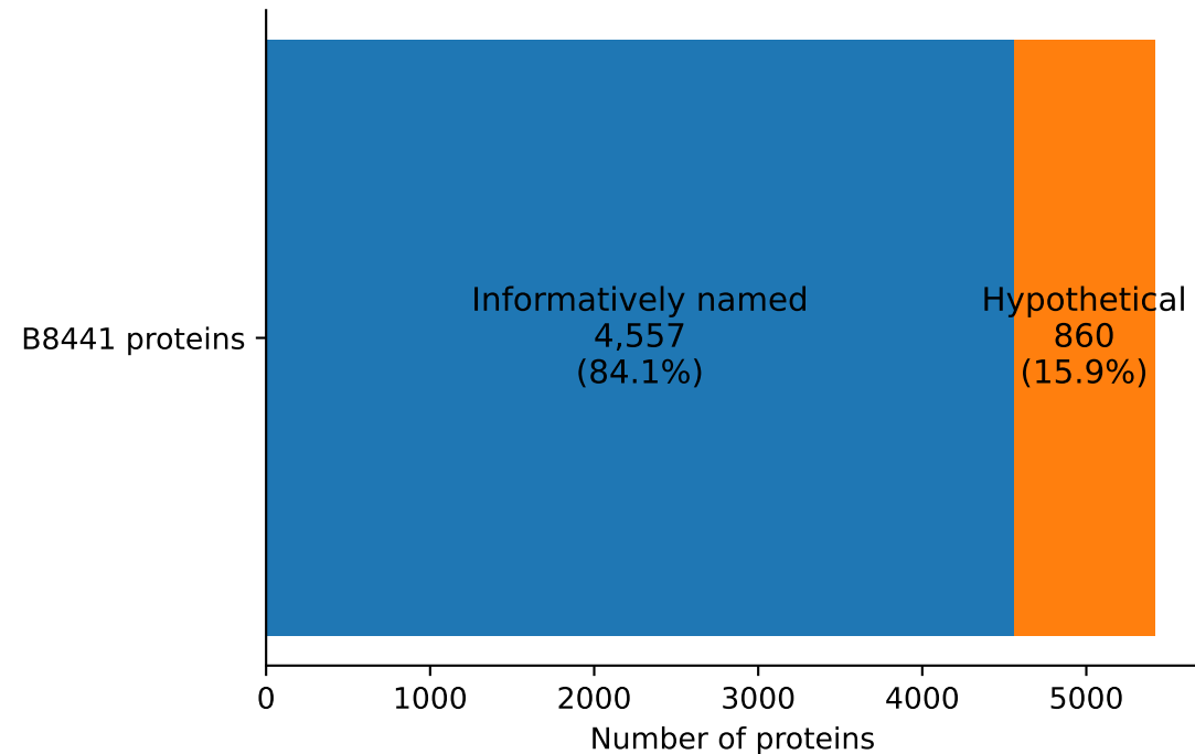
A. Current protein annotation
