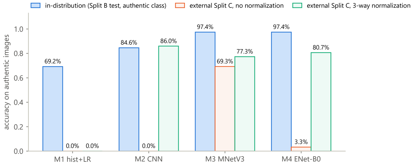
FIGURE S13. In-distribution authentic accuracy against external accuracy before and after three-way normalization, per model, for the run of record. It plots Table 6 of the main paper; M1 bypasses the normalized pipeline by design, so its two Split C bars are the same 0.0% measurement shown twice.
