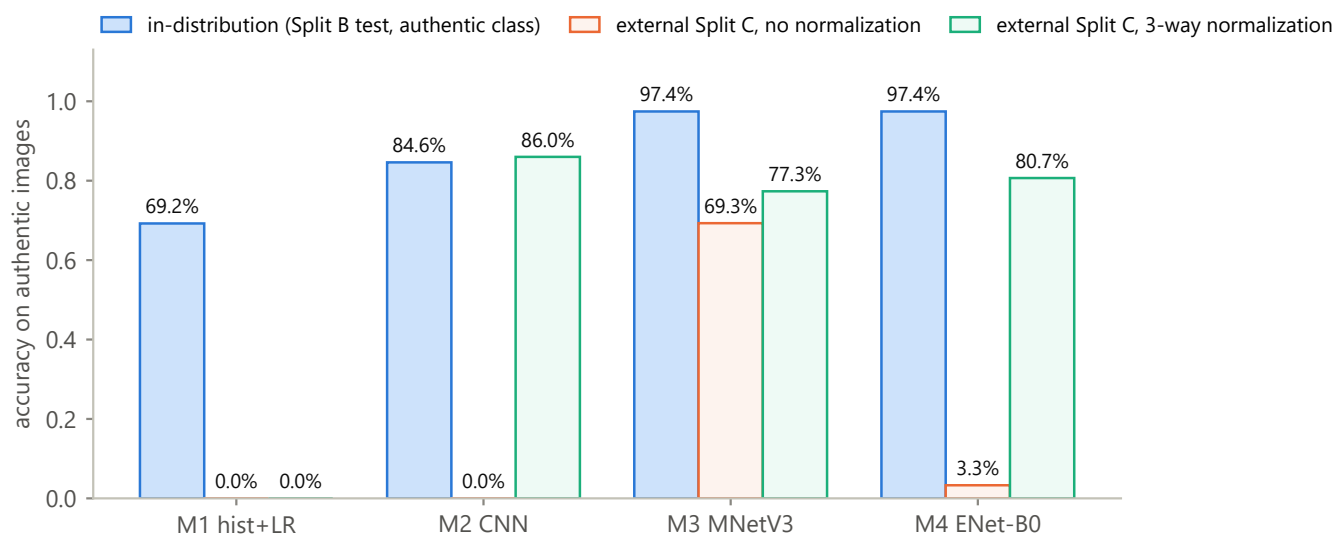
FIGURE S13. In-distribution authentic accuracy against external specificity before and after three-way normalization, per model, for the run of record. It plots Table 4 of the main paper; M1 bypasses the normalized pipeline by design, so its two Split C bars are the same 0.0% measurement shown twice.
