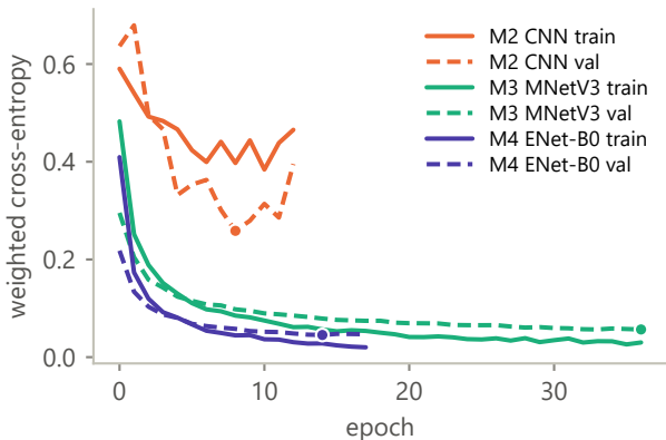
a Loss (solid = train, dashed = val)
