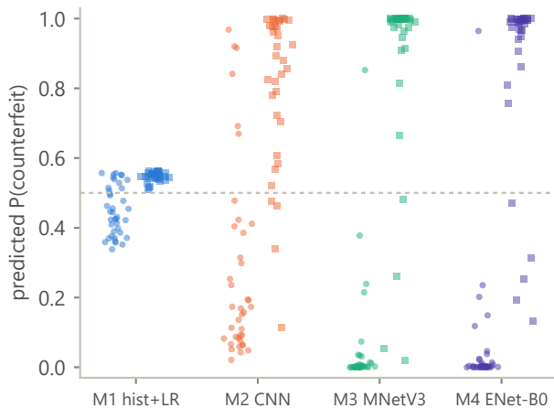
b Score separation ( \circ authentic, \square counterfeit)
