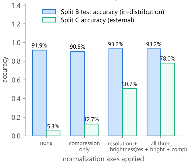
a M4 EfficientNet-B0, single-run ablation
