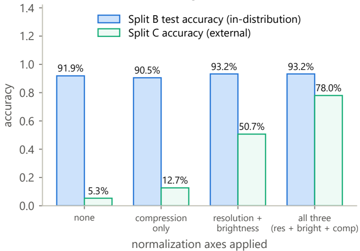
a M4 EfficientNet-B0, single-run ablation
