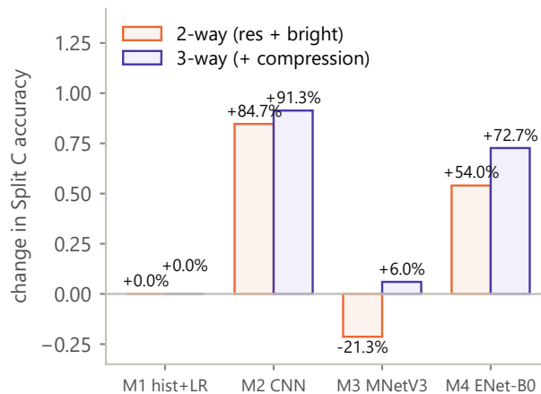
b Which axes help which architecture
