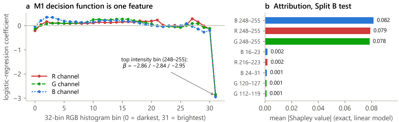
FIGURE S12. (a) M1’s logistic-regression coefficients across the 32 intensity bins of each RGB channel; the near-white bin dominates all three channels. (b) The eight features with the largest mean |Shapley value| on the Split B test partition. Attribution is exact for this model, not sampled. Removing the confound does not unlock latent signal in this model, because there was no latent signal to unlock. We therefore report M1 as a clean negative result: on this benchmark, a classical color-statistics baseline is structurally incapable of the intended task, and its 83.8% accuracy is a measurement of the confound rather than of packaging authenticity. We considered enlarging its feature set (texture descriptors, color moments, edge statistics) and decided against it: the model shows zero external signal across every condition tested in this study, in both external evaluations, and a larger hand-crafted feature set is unlikely to overturn a pattern that is consistent. The negative result is the useful finding.
