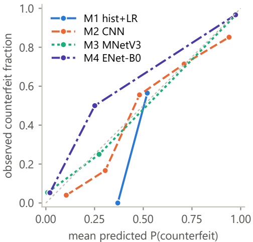
a Reliability, Split B test
