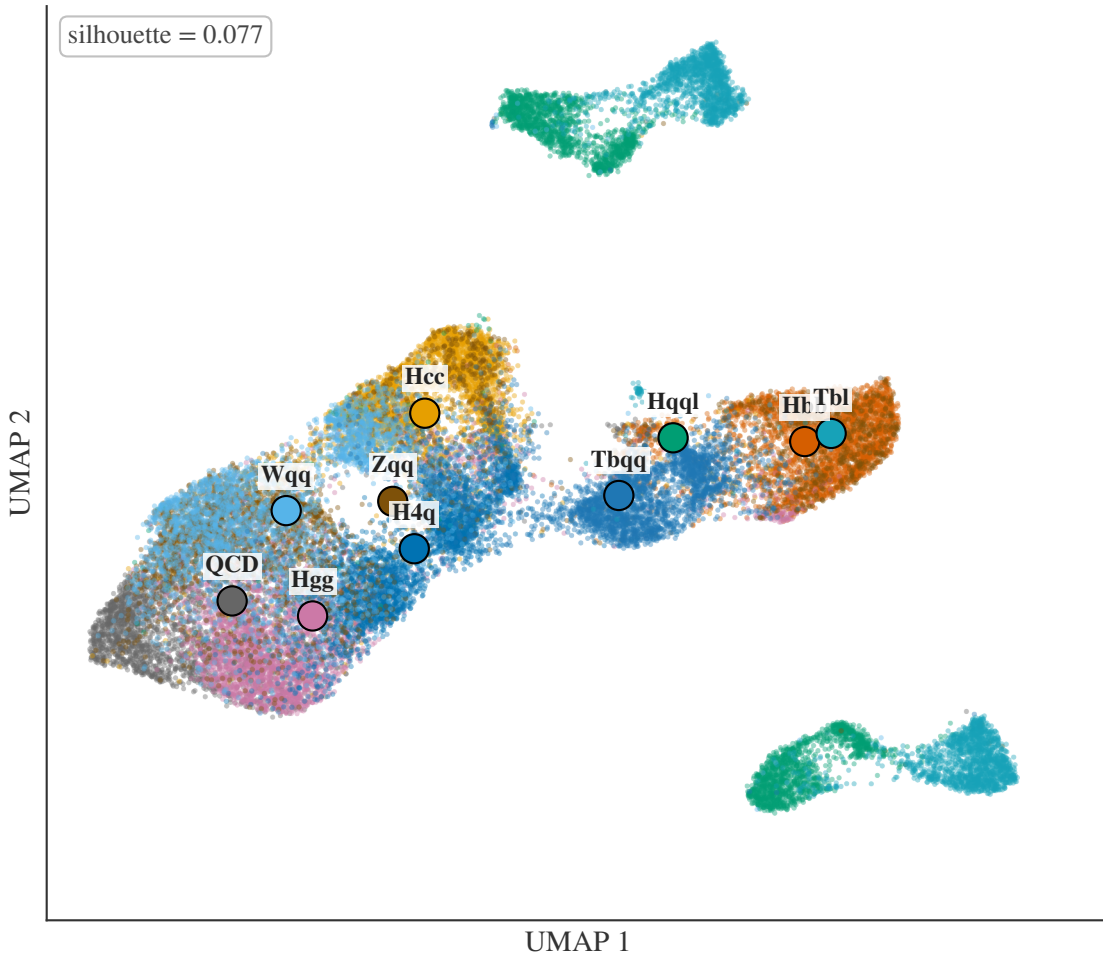
Pretrained Sophon
