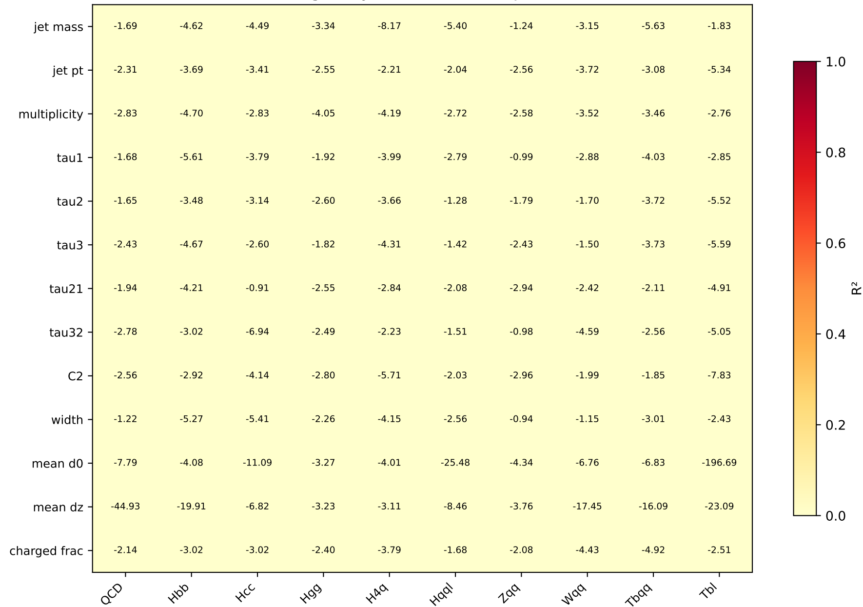
Probing R^2 by Observable and Jet Class
