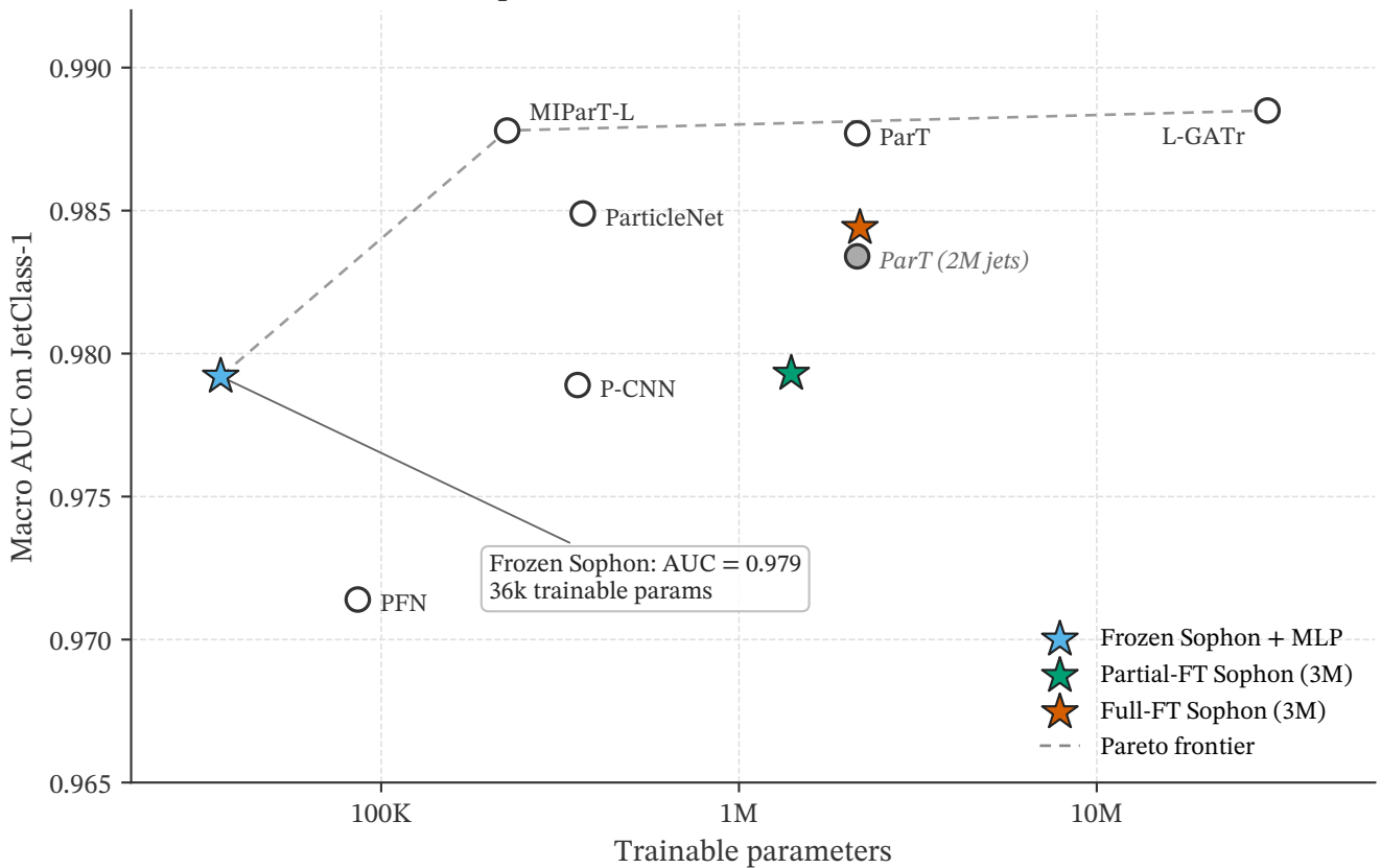
Pareto: parameters vs. AUC on JetClass-1 (10-class)
