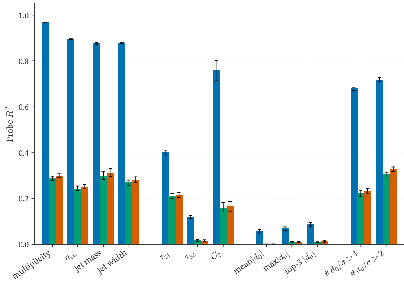
Nonlinear (MLP) probe
