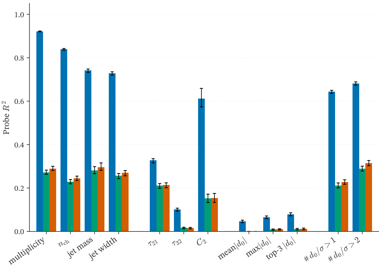
Linear (ridge) probe
