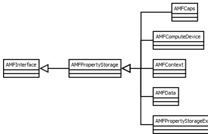
Figure 2 — AMFPropertyStorage inherit diagram
