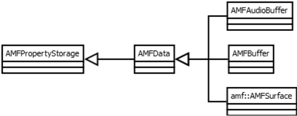
Figure 3 — AMFData inherit diagram
