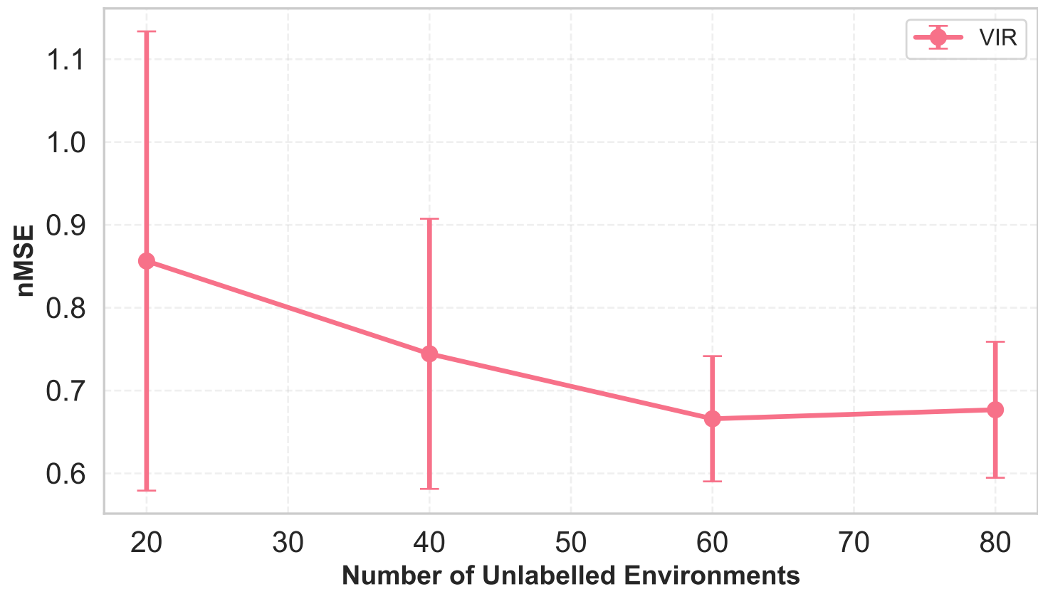
VIR: Effect of Unlabelled Environments
