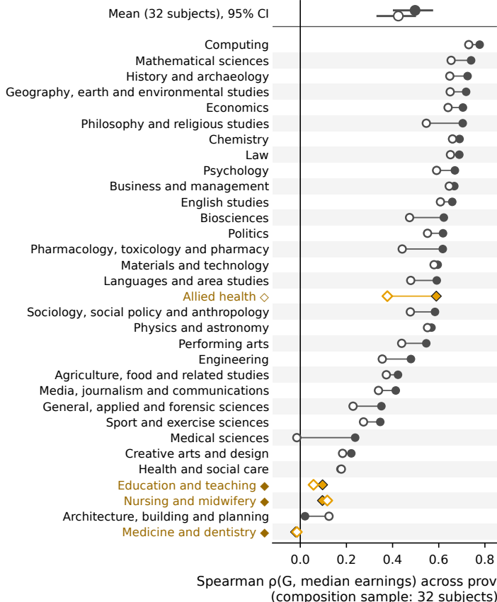
(a) Coupling by subject (UK)
