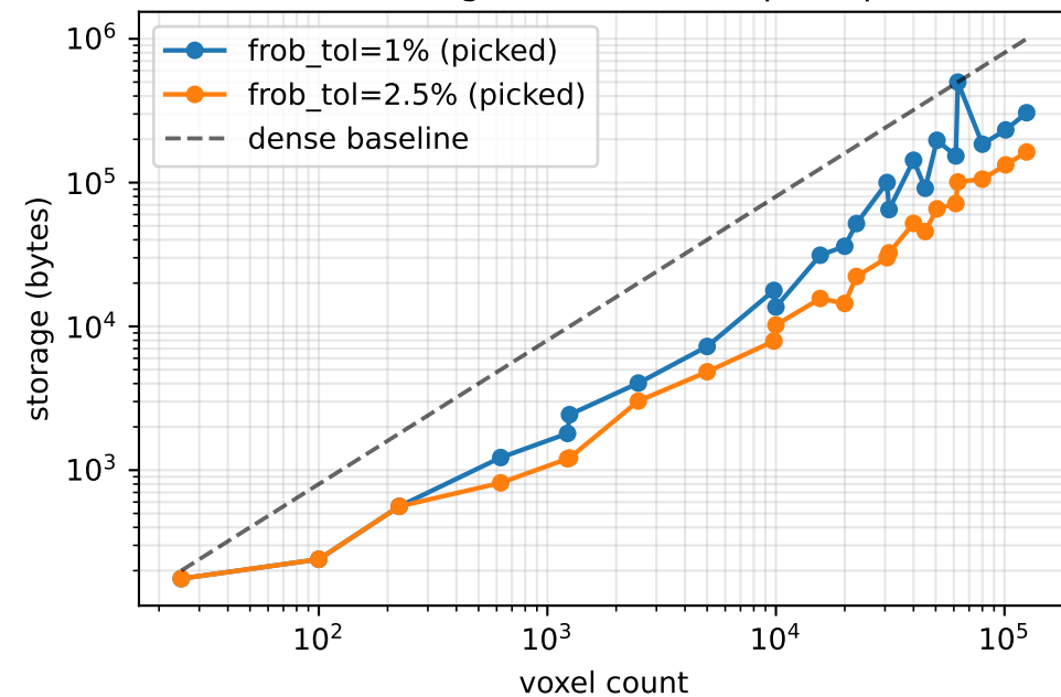
On-disk storage (dense vs adaptive picker)
