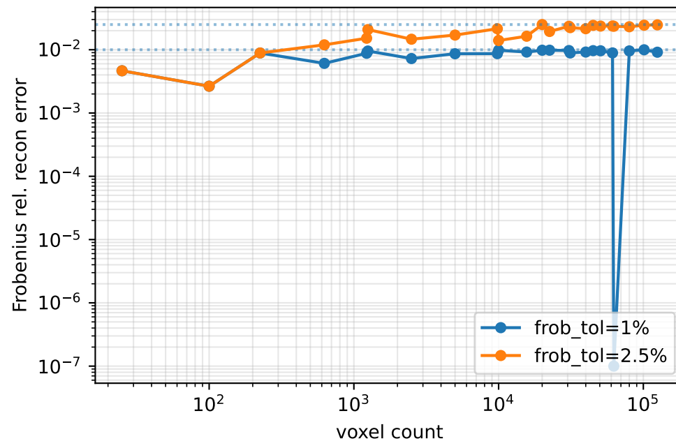
Reconstruction error (dotted = tolerance)
