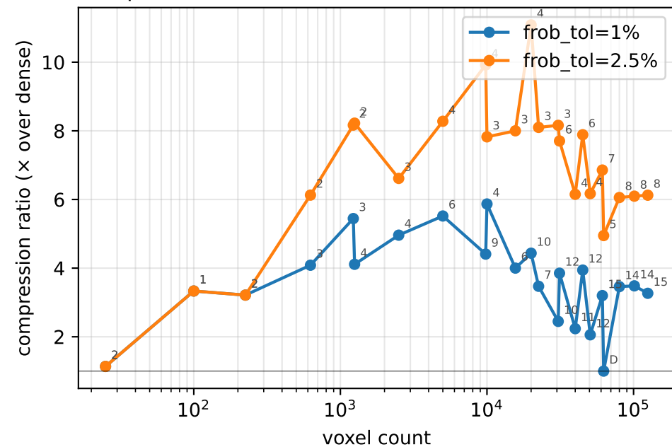
Compression ratio (numbers = SVD rank, D = dense)
