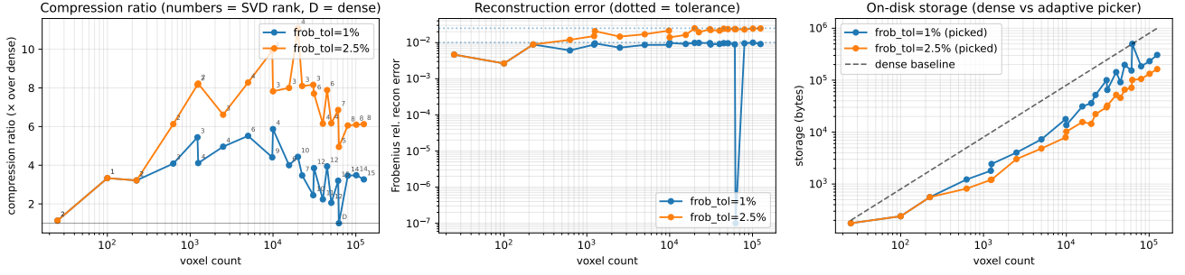
Figure 8. Adaptive SVD compression of the random-ray adjoint flux on the slab benchmark, water at 1 MeV, 1-group, mortal rays ( 200 \times 8000 ). 23 mesh configurations restricted to physically meaningful voxel resolutions (smallest edge \geq \text{mf}/8 \approx 1.77 cm); voxel counts span 25 to 1.25 \times 10^5 . Annotations are SVD rank chosen (D = dense fallback). Left: compression ratio at \varepsilon = 2.5\% rises to \sim 8 – 11\times between 10^3 and 10^5 voxels and stays in that band; the peak is 11.09\times at 20 \times 20 \times 50 = 20\,000 voxels. Middle: linear reconstruction error stays under the requested tolerance band on every retained SVD pick; dense fallbacks are off-scale (exact, plotted at the \varepsilon floor). Right: storage in bytes — picked vs dense.
