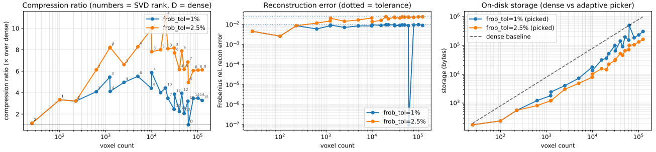
Figure 12. Adaptive SVD compression of the random-ray adjoint flux on the slab benchmark, water at 1 MeV, 1-group, mortal rays (200×8000). 23 mesh configurations restricted to physically meaningful voxel resolutions (smallest edge \geq \text{mf}/8 \approx 1.77 \text{ cm} ); voxel counts span 25 to 1.25 \times 10^5 . Annotations are SVD rank chosen (D = dense fallback). Left: compression ratio at \varepsilon = 2.5\% rises to \sim 8 – 11\times between 10^3 and 10^5 voxels and stays in that band; the peak is 11.09\times at 20 \times 20 \times 50 = 20\,000 voxels. Middle: linear reconstruction error stays under the requested tolerance band on every retained SVD pick; dense fallbacks are off-scale (exact, plotted at the \varepsilon floor). Right: storage in bytes — picked vs dense.
