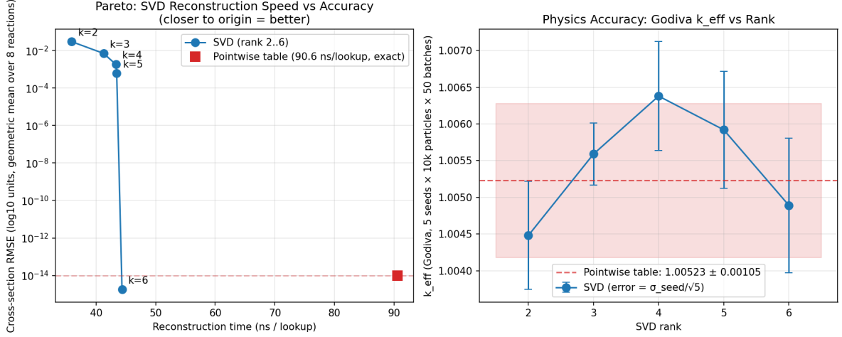
Figure 3: Godiva, laptop. Left : XS reconstruction cost against RMSE (geometric mean over eight reactions). Right : k_{\text{eff}} versus SVD rank, SEM error bars over five seeds. Horizontal band: pointwise-table reference in the same engine.
