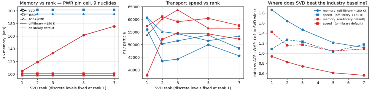
Figure 8. PWR pin cell (9 nuclides, thermal spectrum) sweep across SVD rank \in \{1, 2, 3, 5, 7\} . Left : on-library SVD memory crosses the table line at every rank; off-library table memory ( \sim 200 MB) dominates because pseudo-interpolation must keep both T -bracket columns resident. Centre : ns/particle on PWR is dominated by physics work (thousands of collisions per history through the U-238 RRR); the rank impact on speed is small. Right : ratio vs ACE+WMP. The off-library memory ratio reaches 1.32\times at rank 5, monotonically decreasing as rank increases. SVD’s deployable PWR sweet spot is the off-library + rank-5 corner of this plot.
