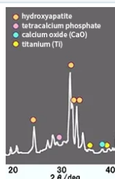
FIG. 02 / CONVENTIONAL HA / XRD
