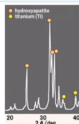
FIG. 04 / AQB RE-CRYSTALLIZED HA / XRD
