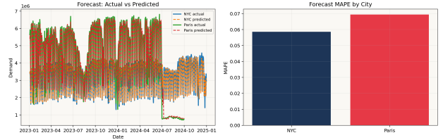
Figure 3: Forecast quality from the current result set.
