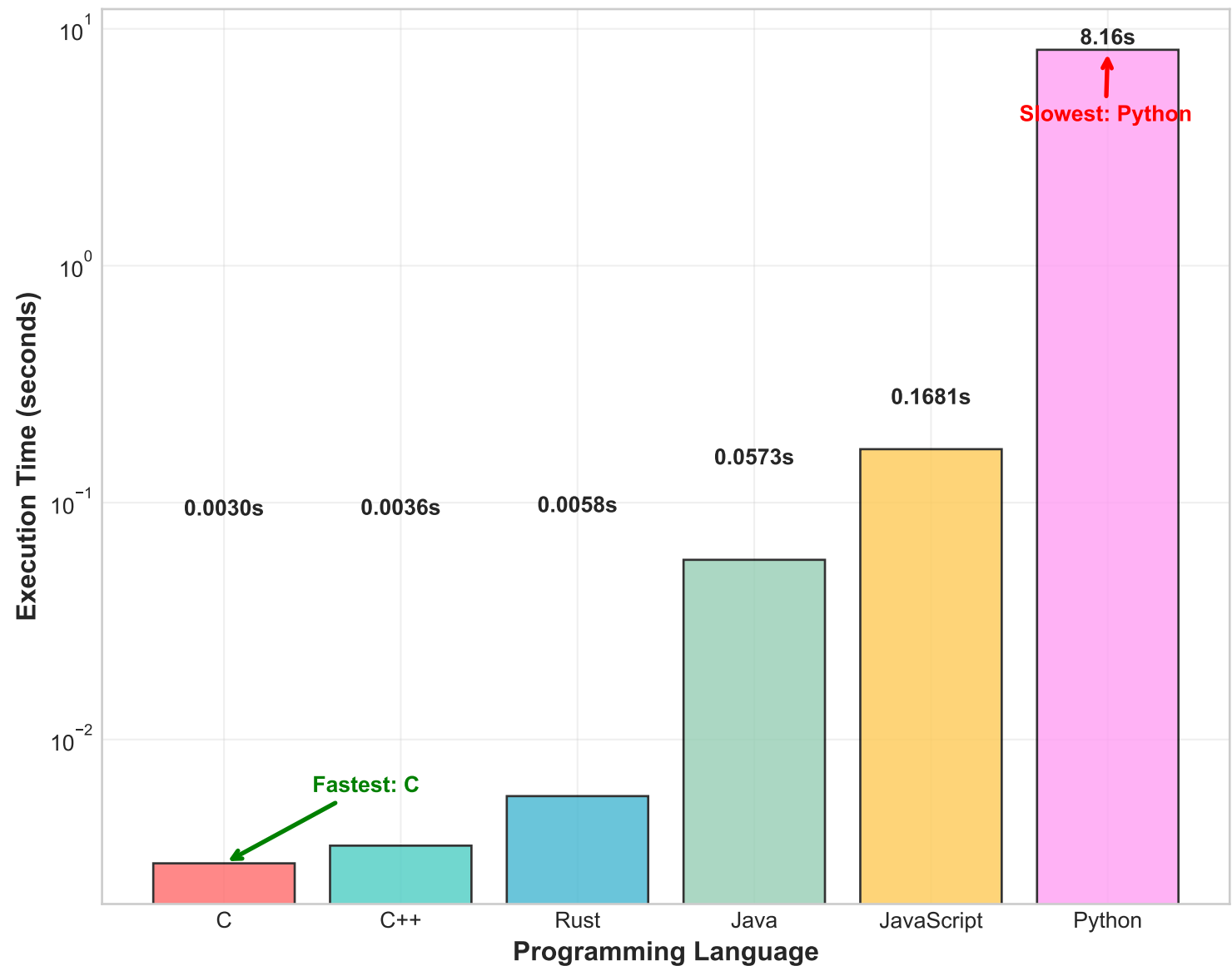
Parallel Matrix Multiplication Performance Comparison (500×500 matrices, 8 threads)
