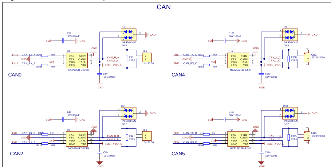
Figure 3-7. Schematic diagram of CAN
