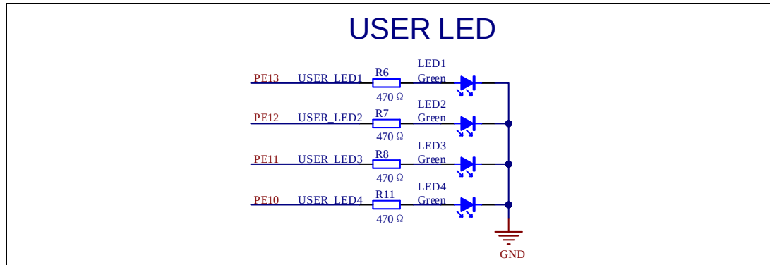
Figure 3-3. Schematic diagram of LED function
