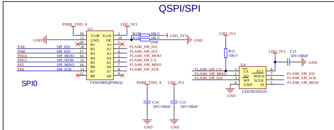
Figure 3-12. Schematic diagram of SPI flash
