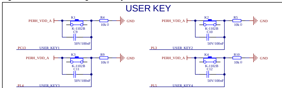
Figure 3-4. Schematic diagram of Key function
