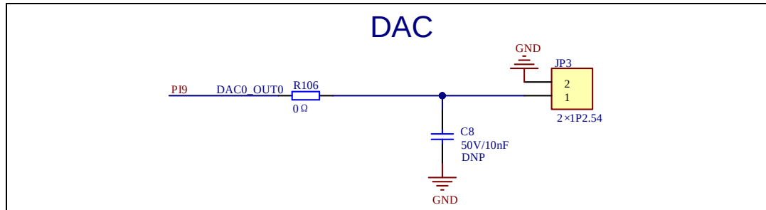
Figure 3-6. Schematic diagram of DAC
