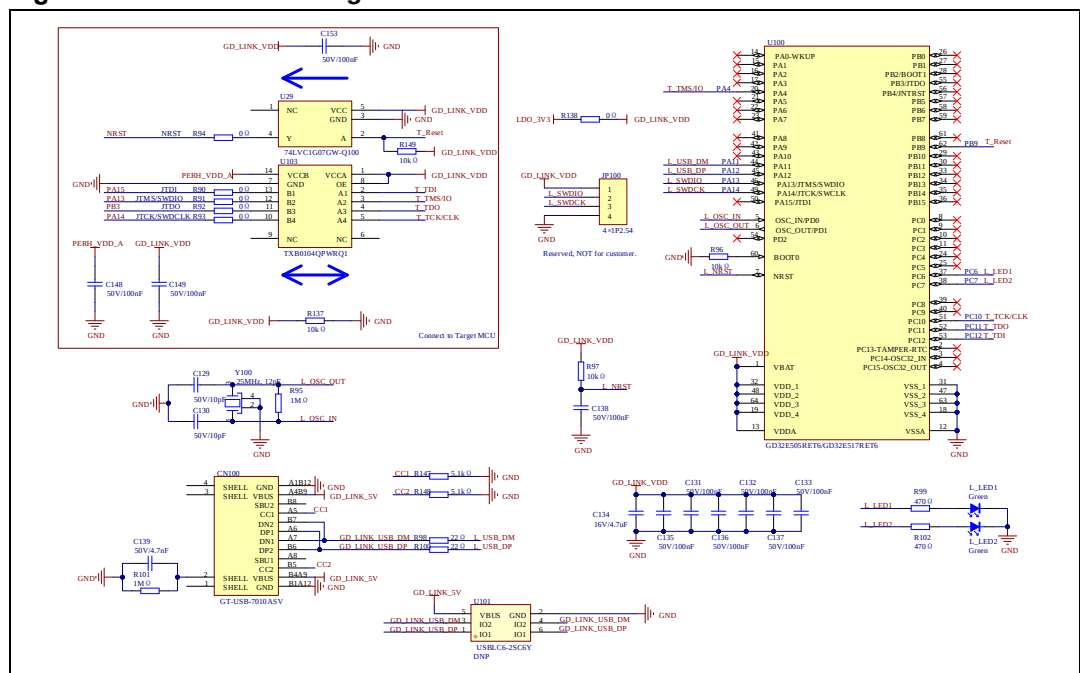
Figure 3-15. Schematic diagram of GD-Link
