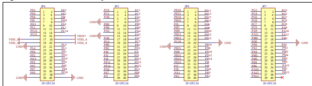
Figure 3-14. Schematic diagram of Extension
