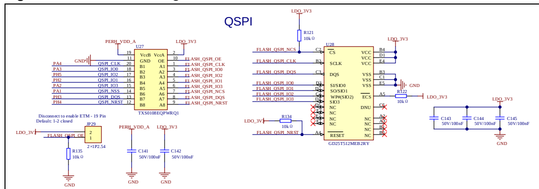
Figure 3-11. Schematic diagram of QSPI
