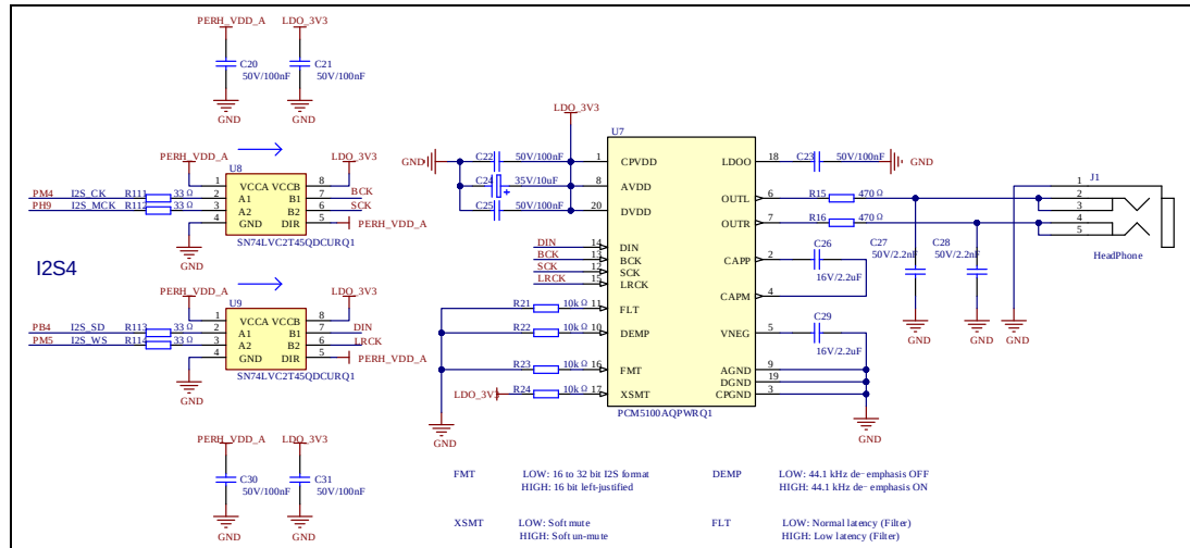
Figure 3-10. Schematic diagram of I2S
