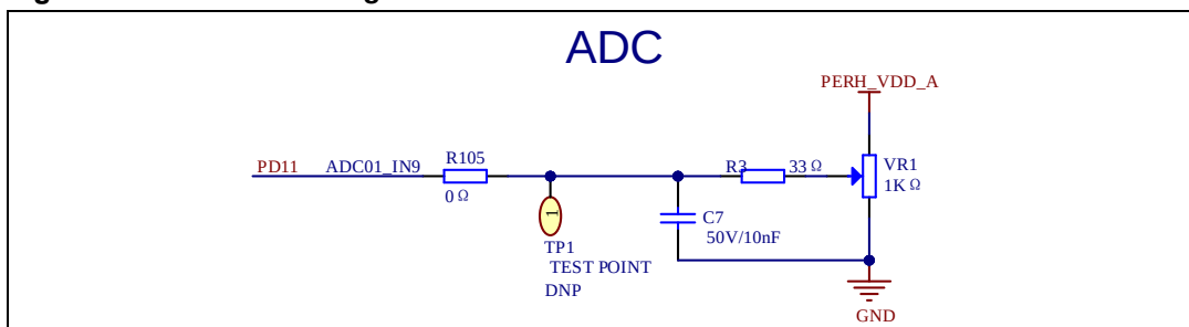
Figure 3-5. Schematic diagram of ADC
