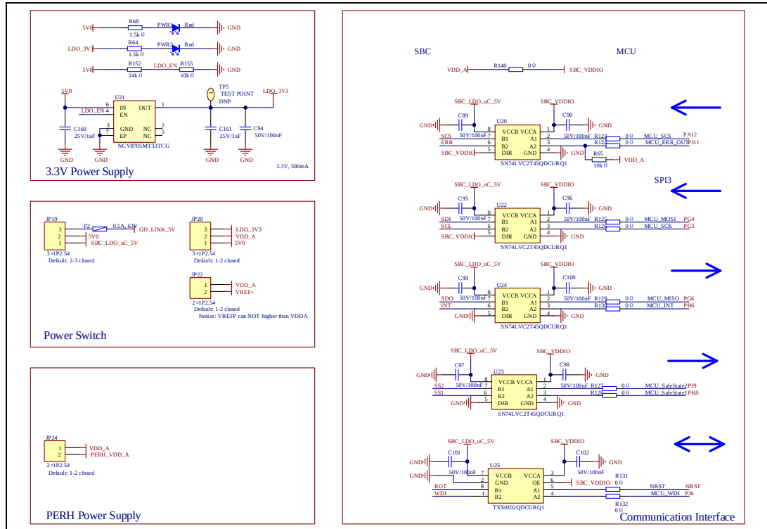
Figure 3-1. Schematic diagram of power supply
