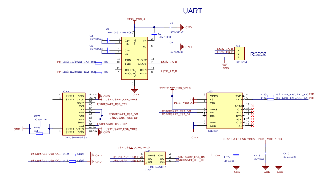
Figure 3-13. Schematic diagram of UART
