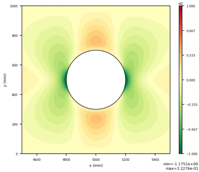
Figure 20. undeformed zoom \sigma_2 .
