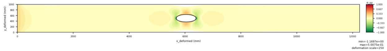
Figure 30. deformed \sigma_{yy} .
