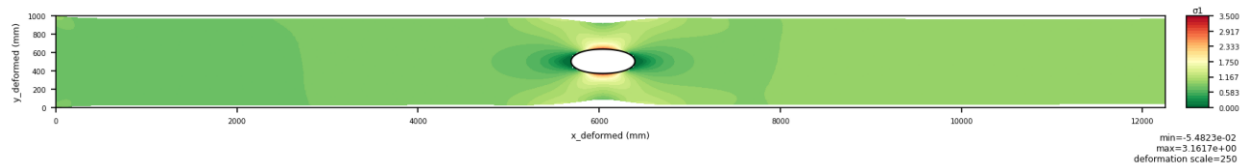
Figure 32. deformed \sigma_1 .
