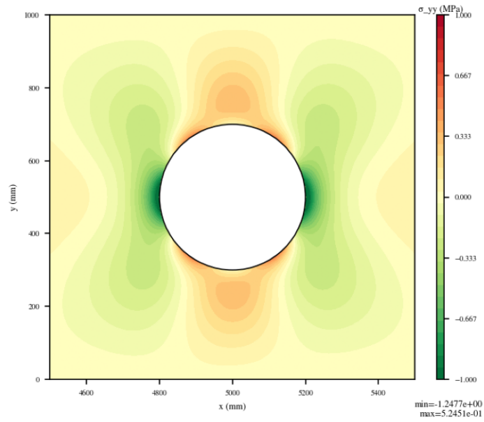
Figure 17. undeformed zoom \sigma_{yy} .
