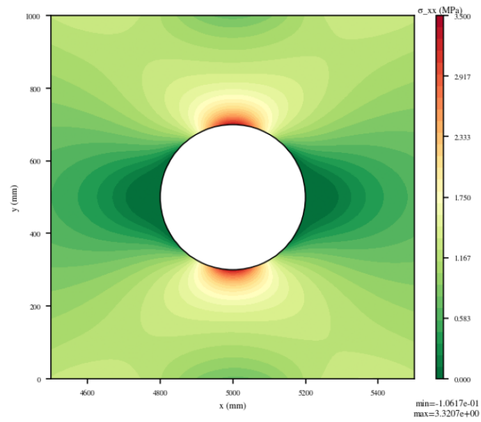
Figure 16. undeformed zoom \sigma_{xx} .
