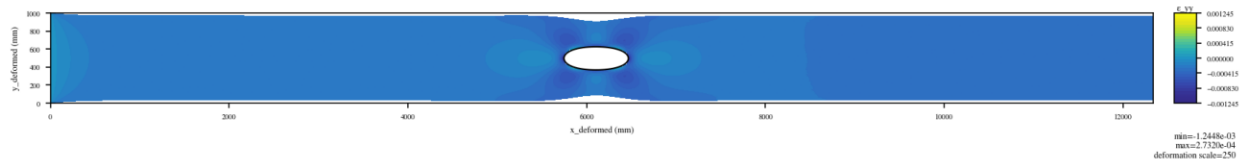
Figure 35. deformed \epsilon_{yy} .
