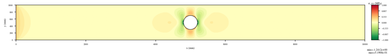
Figure 7. undeformed \sigma_{yy} .
