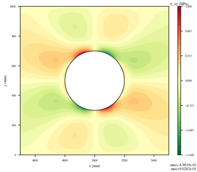
Figure 18. undeformed zoom \sigma_{xy} .
