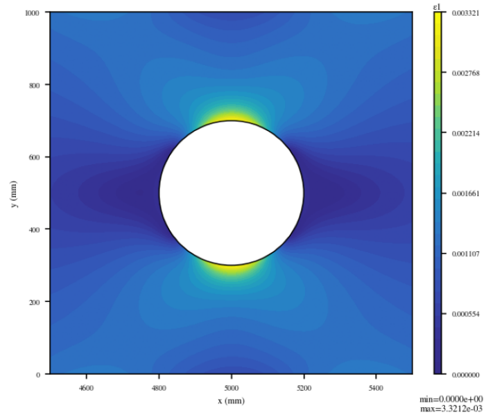
Figure 24. undeformed zoom \epsilon_l .
