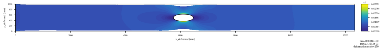
Figure 37. deformed \epsilon_1 .
