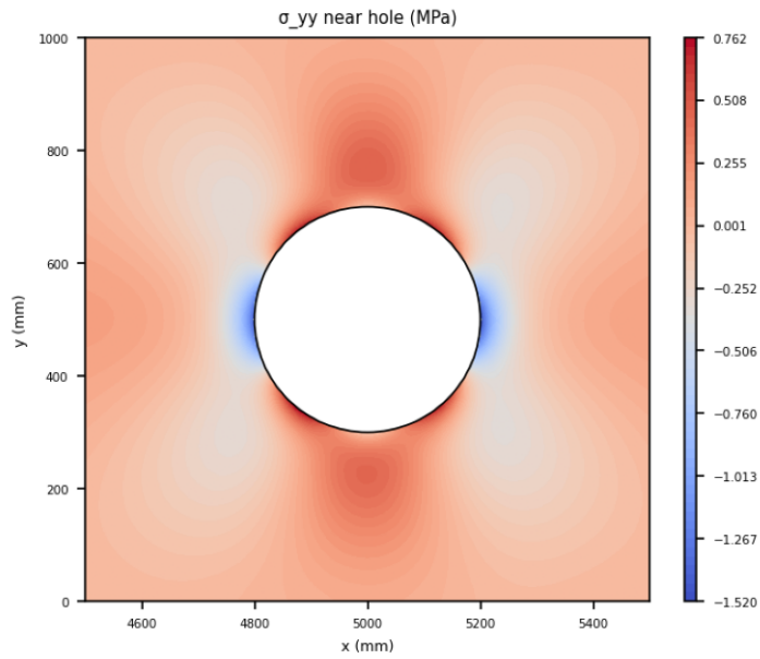
Figure 9. \sigma_{yy} near hole (MPa) - near-hole detail.
