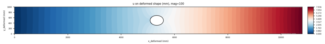
Figure 11. Deformed x -displacement field.
