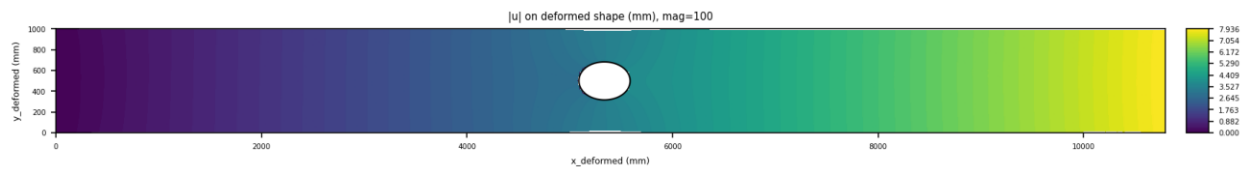
Figure 13. Deformed displacement-magnitude field.
