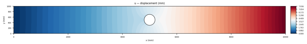
Figure 3. x -displacement u (mm).
