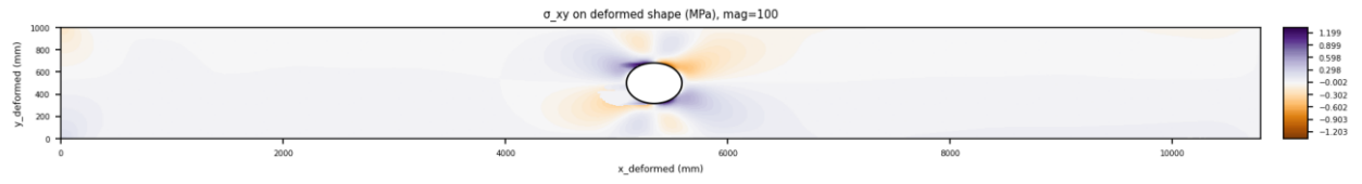
Figure 16. Deformed \tau_{xy} field.
