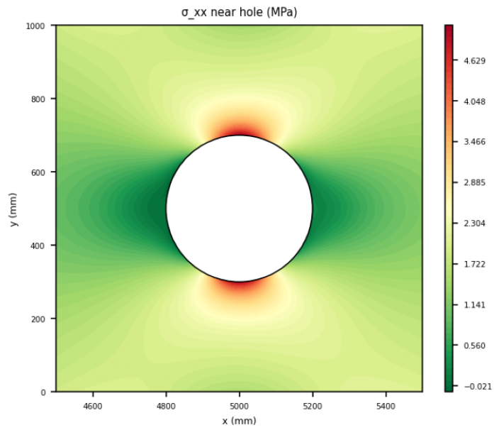
Figure 8. \sigma_{xx} near hole (MPa) - near-hole detail.
