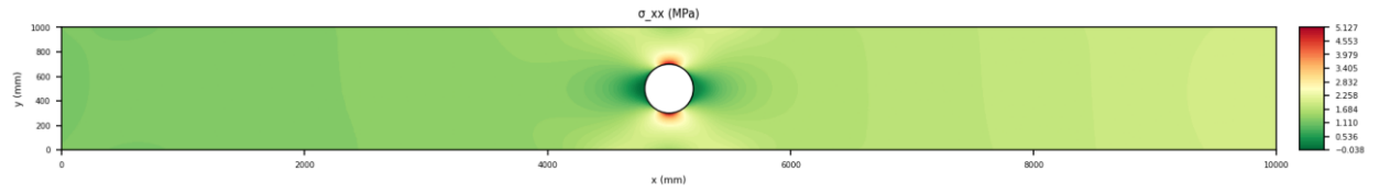
Figure 5. \sigma_{xx} (MPa).
