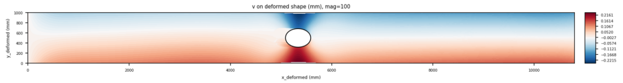
Figure 12. Deformed y -displacement field.
