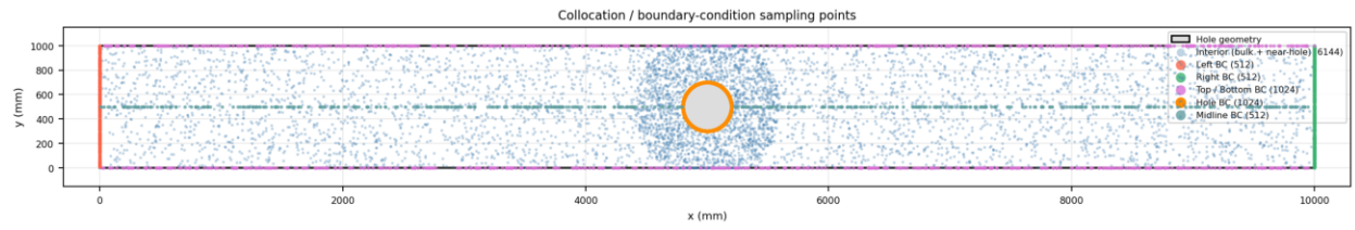
Figure 1. Training collocation points, including near-hole enrichment and boundary sampling.
