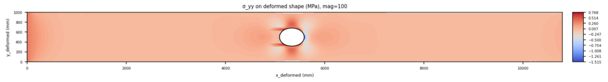
Figure 15. Deformed \sigma_{yy} field.
