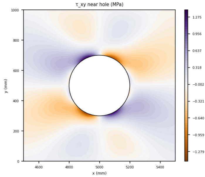
Figure 10. \tau_{xy} near hole (MPa) - near-hole detail.
