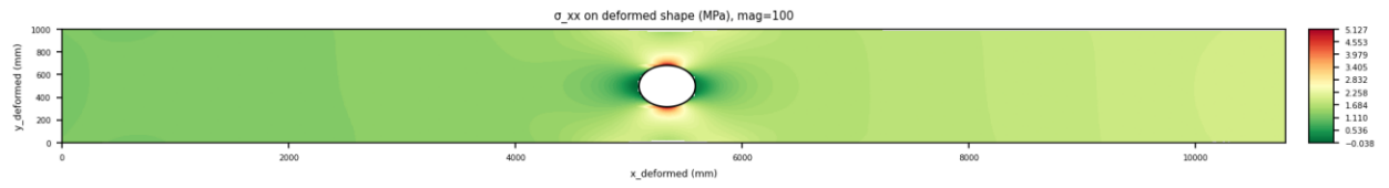
Figure 14. Deformed \sigma_{xx} field.
