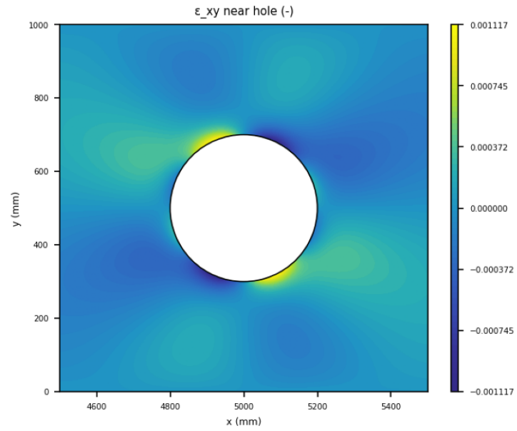
Figure 23. undeformed zoom \epsilon_{xy} .
