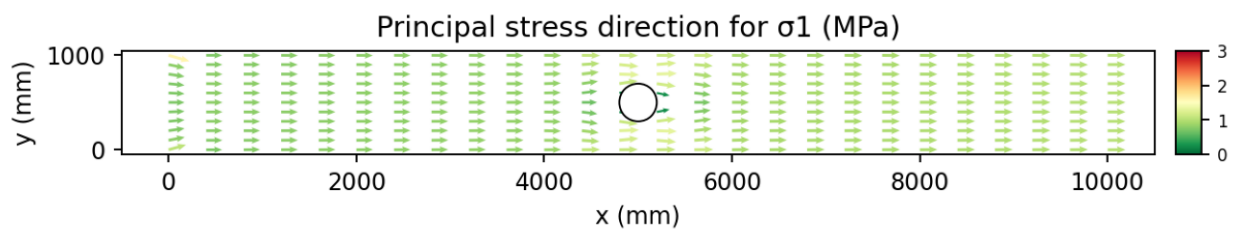
Figure 39. undeformed vector \sigma_1 .
