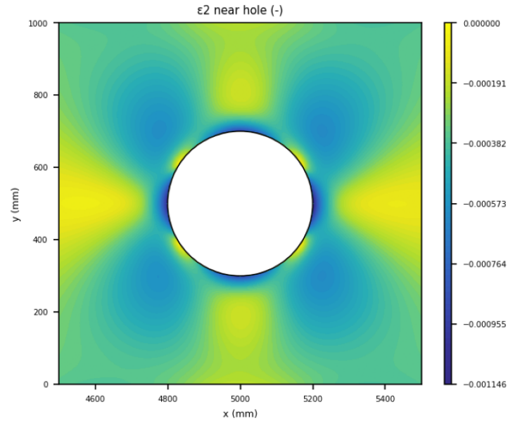
Figure 25. undeformed zoom \epsilon_2 .
