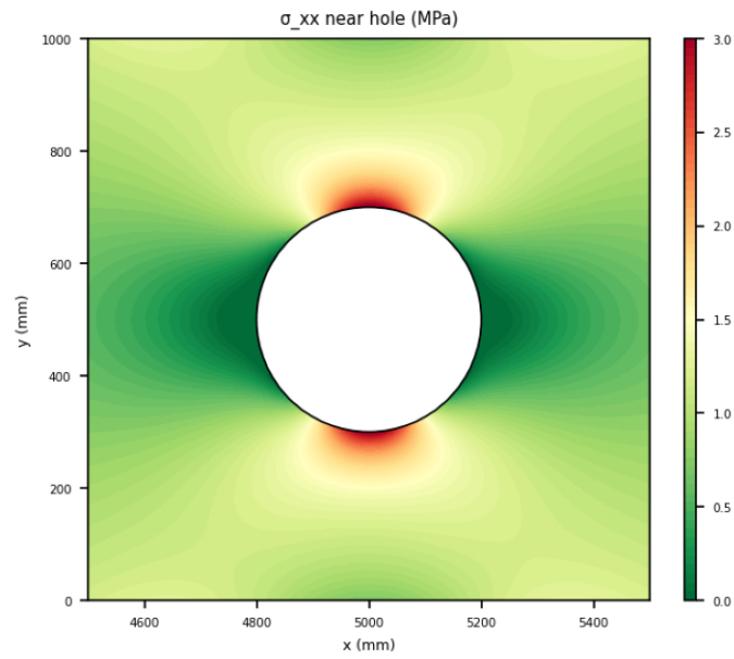
Figure 16. undeformed zoom \sigma_{xx} .
