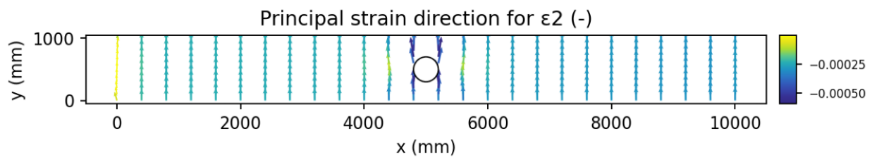
Figure 42. undeformed vector \epsilon_2 .
