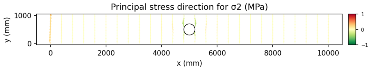
Figure 40. undeformed vector \sigma_2 .
