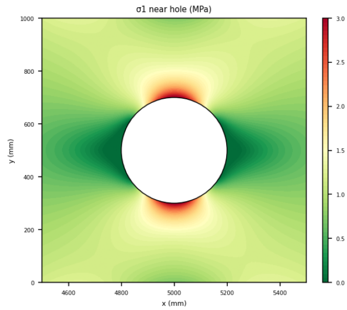
Figure 19. undeformed zoom \sigma_1 .
