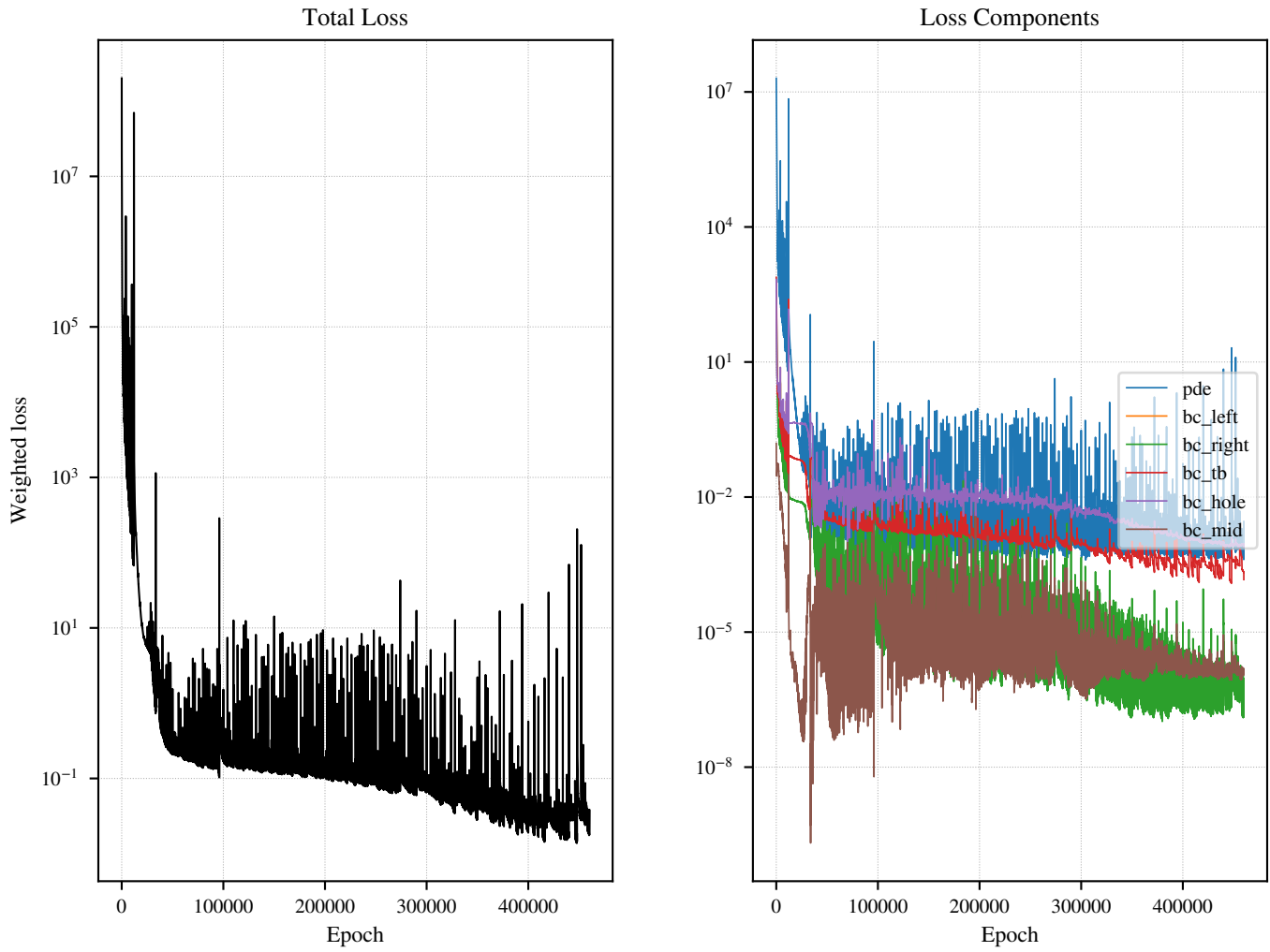
Figure 2. Training loss history on a log scale. Left: total weighted loss. Right: individual PDE and boundary loss components.
