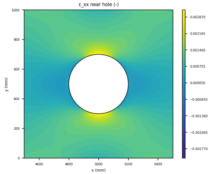
Figure 21. undeformed zoom \epsilon_{xx} .
