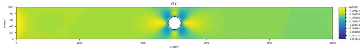
Figure 15. undeformed \epsilon_2 .
