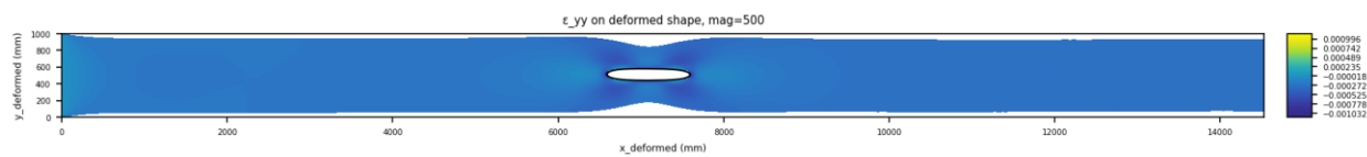
Figure 35. deformed \varepsilon_{yy} .
