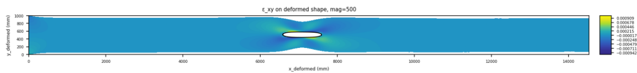
Figure 36. deformed \varepsilon_{xy} .
