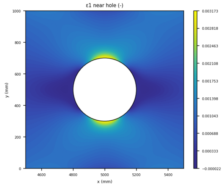
Figure 24. undeformed zoom \epsilon_1 .
