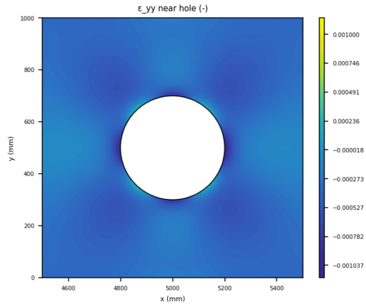
Figure 22. undeformed zoom \epsilon_{yy} .
