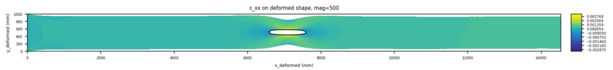
Figure 34. deformed \epsilon_{xx} .
