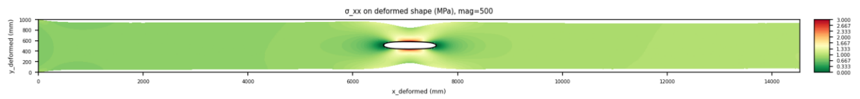
Figure 29. deformed \sigma_{xx} .
