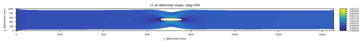
Figure 37. deformed \varepsilon_1 .
