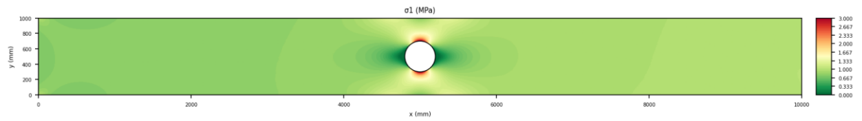
Figure 12. undeformed \sigma_1 .
