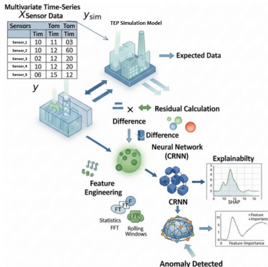
Fig. 4. Physics-based residual generation and anomaly detection pipeline. Measured process observations y_t are compared with nominal TEP simulator predictions \hat{y}_t to compute residuals r_t = y_t - \hat{y}_t using Eq. (3). The residual sequence is then combined with compact engineered descriptors and provided to the proposed CRNN for anomaly probability estimation.
