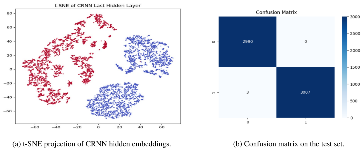
Fig. 8. Representation quality and classification behavior of the proposed physics-guided CRNN learned from residual-enriched inputs.
