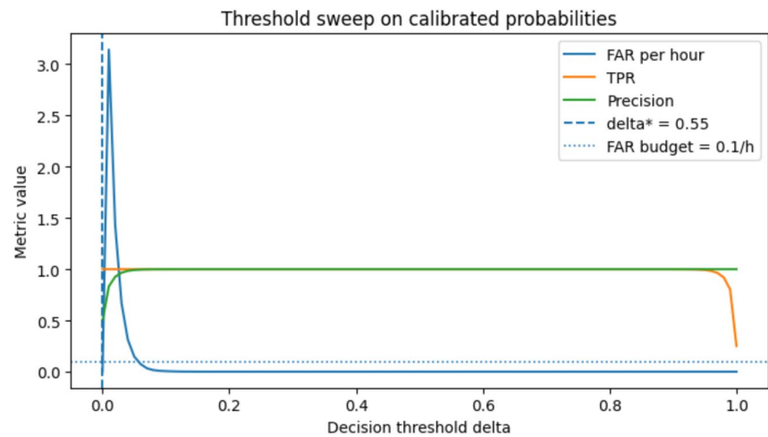
Fig. 12. Threshold-sensitivity analysis on calibrated probabilities. The horizontal axis shows the decision threshold \delta \in [0, 1] and the vertical axis shows the corresponding metric values for \text{FAR}_{\text{hour}}(\delta) , \text{TPR}(\delta) and precision. The dashed vertical line marks the selected operating threshold \delta^* = 0.55 , obtained from Eq. (29) and the dotted horizontal line marks the false-alarm budget \tau_{\text{FAR}} = 0.1 \text{ h}^{-1} from Eq. (30).
