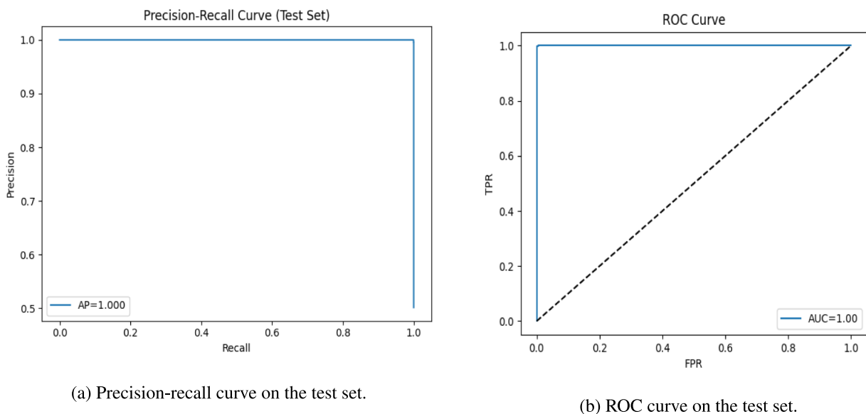
Fig. 9. Discrimination diagnostics for the proposed physics-guided CRNN under the protocol in Algorithm 1.
