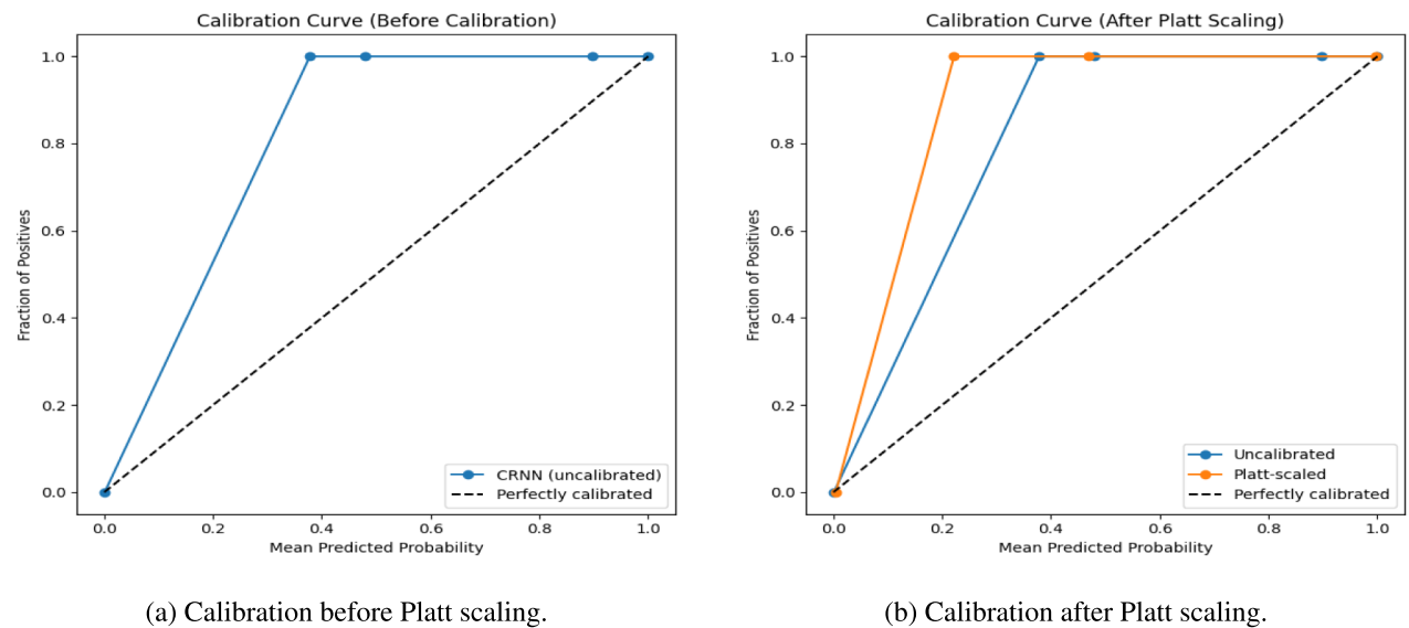
Fig. 11. Probability calibration behavior before and after applying Eq. (18).
