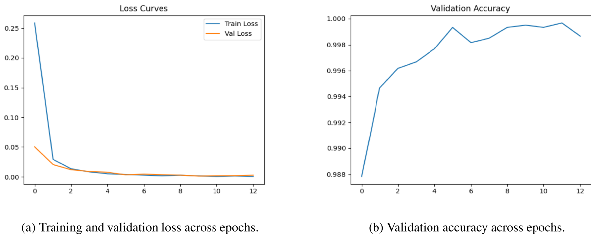
Fig. 7. Optimization dynamics for the proposed physics-guided CRNN under the run-level split in “Dataset and split”.
