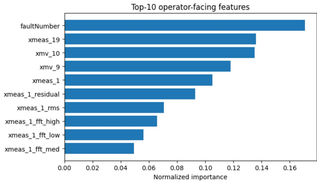
Fig. 14. Global top-10 operator-facing feature-importance summary under the SHAP-guided selection procedure in “Feature construction and SHAP-guided selection”. Unlike Fig. 13, which shows local fault-specific explanations, this figure ranks the features that contribute most consistently across the evaluation set.
