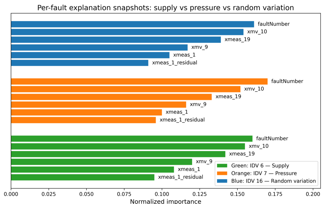
Fig. 13. Representative per-fault local explanation snapshots for selected fault families. Each color-coded block corresponds to one selected fault example and shows the channels and descriptors that contribute most strongly to the corresponding alarm decision. Exact fault IDs and families are indicated in the legend.
