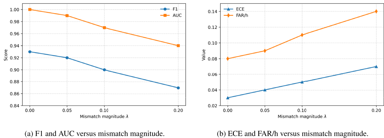
Fig. 15. Performance under controlled reference-model mismatch. The horizontal axis shows the mismatch magnitude \lambda defined in Eq. (31). Panel (a) shows progressive degradation in F1 and AUC as mismatch increases, while panel (b) shows worsening calibration and increased nuisance alarms through ECE and FAR/h.
