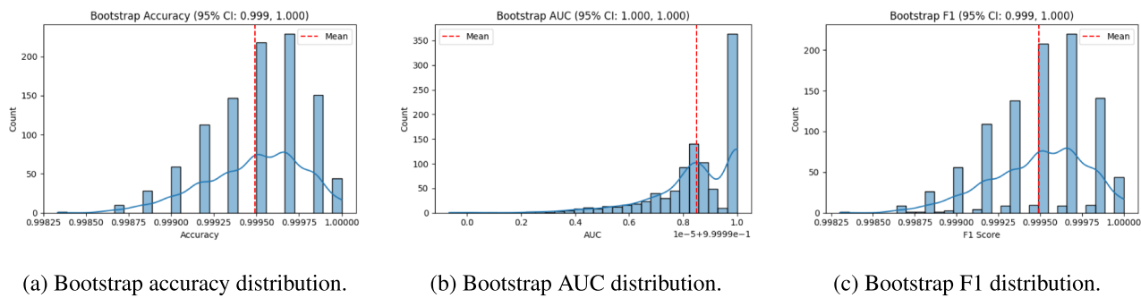
Fig. 10. Bootstrap reliability of discrimination metrics using the BCa procedure in Eq. (35).
