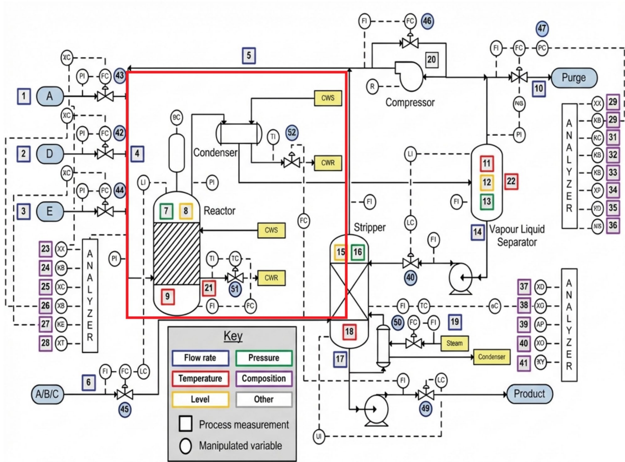
Fig. 3. Tennessee Eastman Process schematic with the highlighted region of interest. The red box marks the reactor-condenser recycle loop and its associated feed and utility interactions, where coupled dynamics, operating-mode changes and sensor correlations often cause subtle drifts and delayed fault effects that are difficult to govern with fixed thresholds. The schematic is adapted and enhanced from the original Tennessee Eastman Process diagram reported in 42 .
